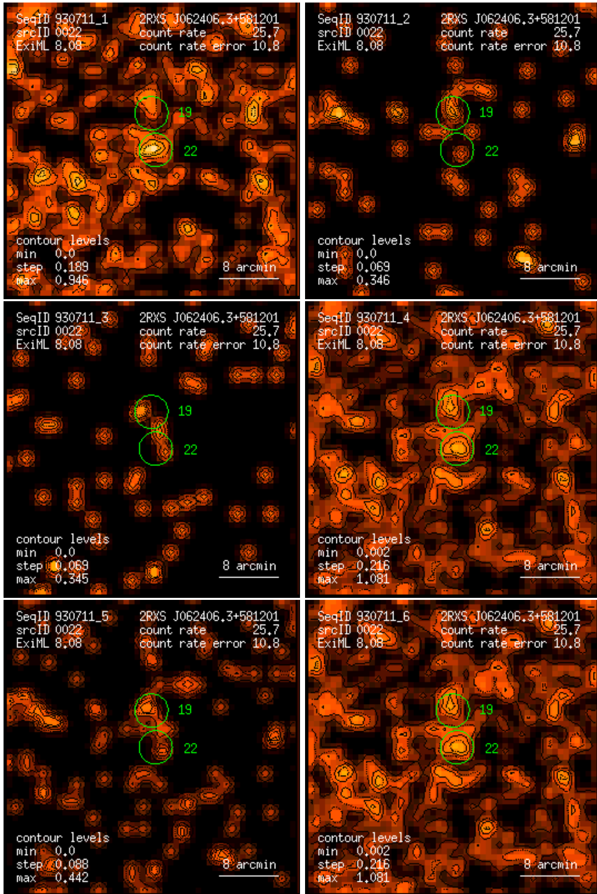
Figure 22: RASS 930711: detection 0022: band rate images, Gaussian filter: (1) PSPC channels 11 – 41, (2) 52 – 90, (3) 91 – 201, (4) 11 – 235, (5) 52 – 201, (6) 11 – 201. Broad band rates in counts/ks. Band rate contour levels in counts/ks/arcmin 2 .
