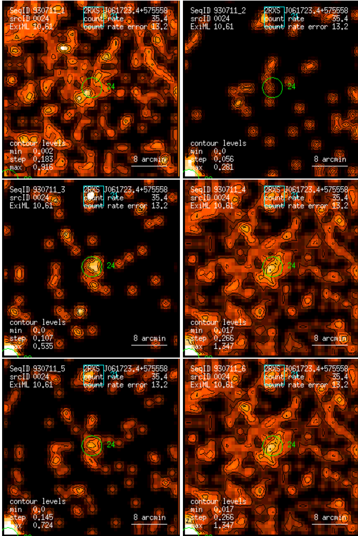
Figure 24: RASS 930711: detection 0024: band rate images, Gaussian filter: (1) PSPC channels 11 – 41, (2) 52 – 90, (3) 91 – 201, (4) 11 – 235, (5) 52 – 201, (6) 11 – 201. Broad band rates in counts/ks. Band rate contour levels in counts/ks/arcmin 2 .
