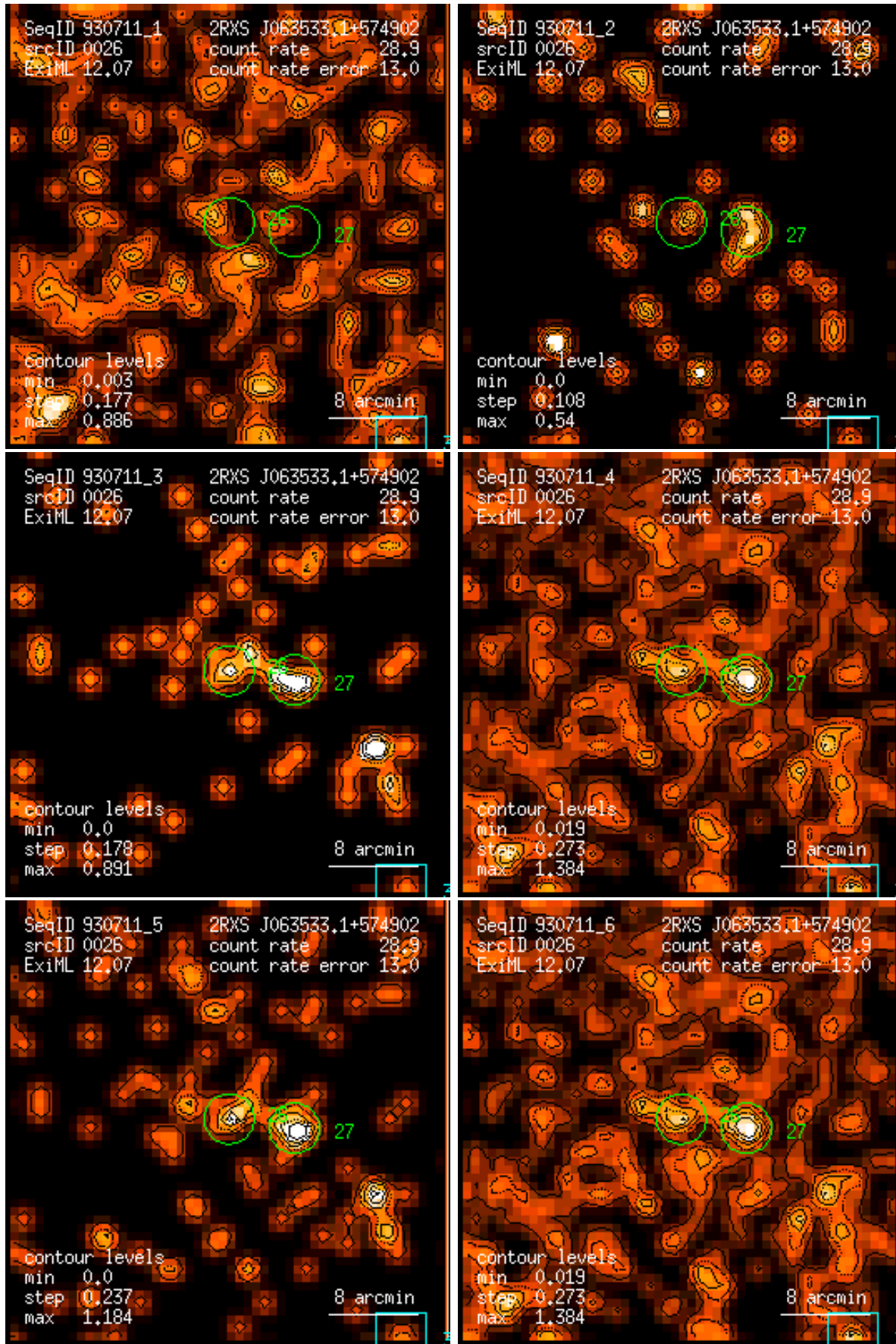
Figure 26: RASS 930711: detection 0026: band rate images, Gaussian filter: (1) PSPC channels 11 – 41, (2) 52 – 90, (3) 91 – 201, (4) 11 – 235, (5) 52 – 201, (6) 11 – 201. Broad band rates in counts/ks. Band rate contour levels in counts/ks/arcmin 2 .
