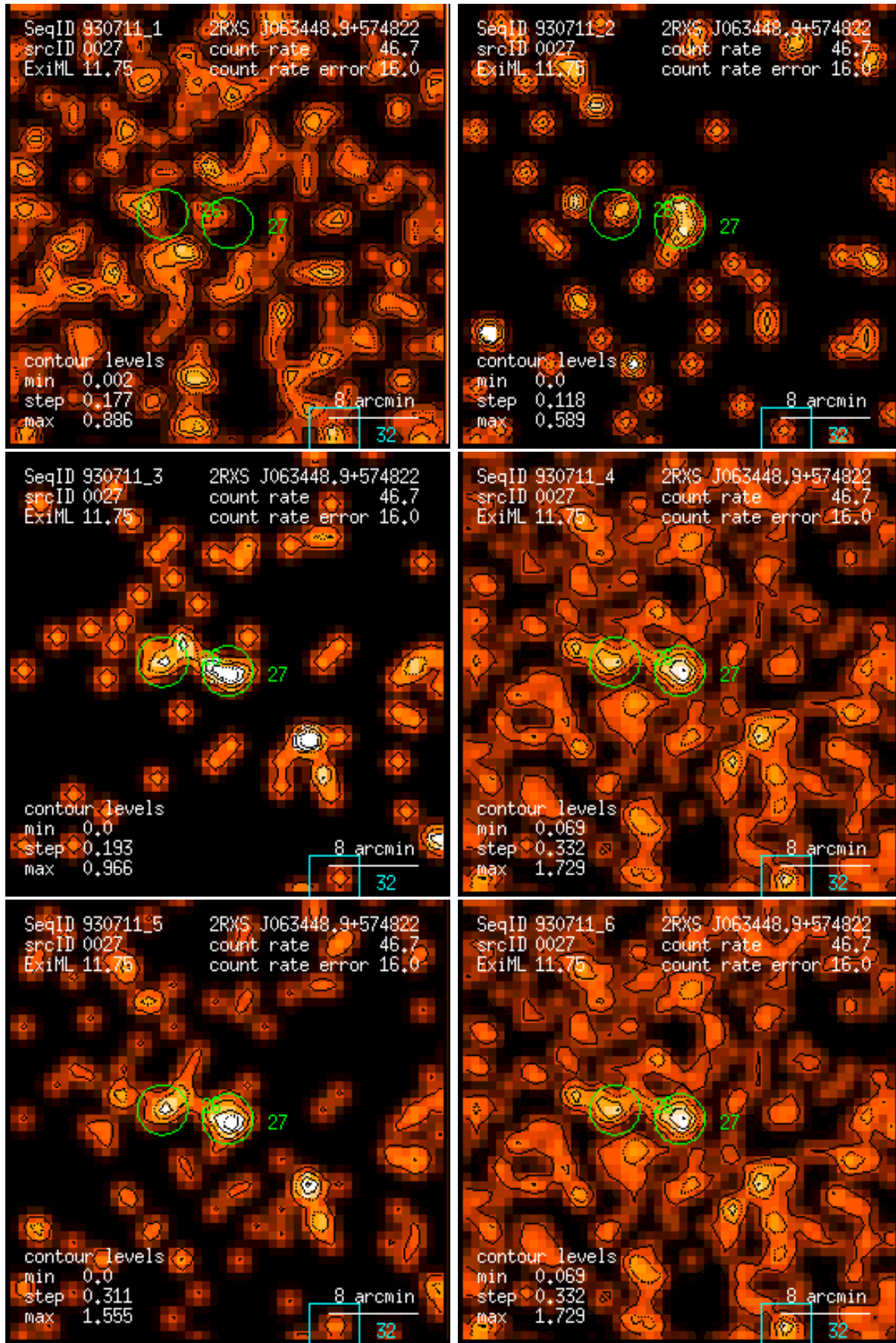
Figure 27: RASS 930711: detection 0027: band rate images, Gaussian filter: (1) PSPC channels 11 – 41, (2) 52 – 90, (3) 91 – 201, (4) 11 – 235, (5) 52 – 201, (6) 11 – 201. Broad band rates in counts/ks. Band rate contour levels in counts/ks/arcmin 2 .
