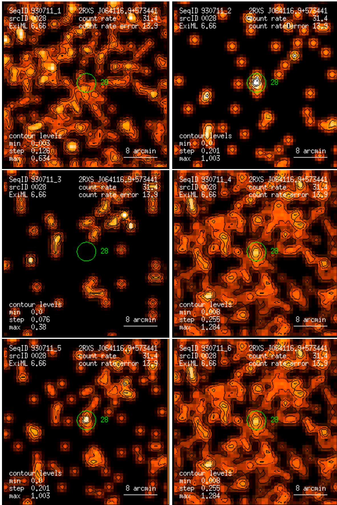
Figure 28: RASS 930711: detection 0028: band rate images, Gaussian filter: (1) PSPC channels 11 – 41, (2) 52 – 90, (3) 91 – 201, (4) 11 – 235, (5) 52 – 201, (6) 11 – 201. Broad band rates in counts/ks. Band rate contour levels in counts/ks/arcmin 2 .
