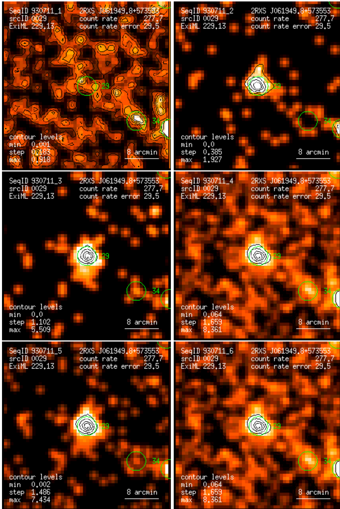
Figure 29: RASS 930711: detection 0029: band rate images, Gaussian filter: (1) PSPC channels 11 – 41, (2) 52 – 90, (3) 91 – 201, (4) 11 – 235, (5) 52 – 201, (6) 11 – 201. Broad band rates in counts/ks. Band rate contour levels in counts/ks/arcmin 2 .
