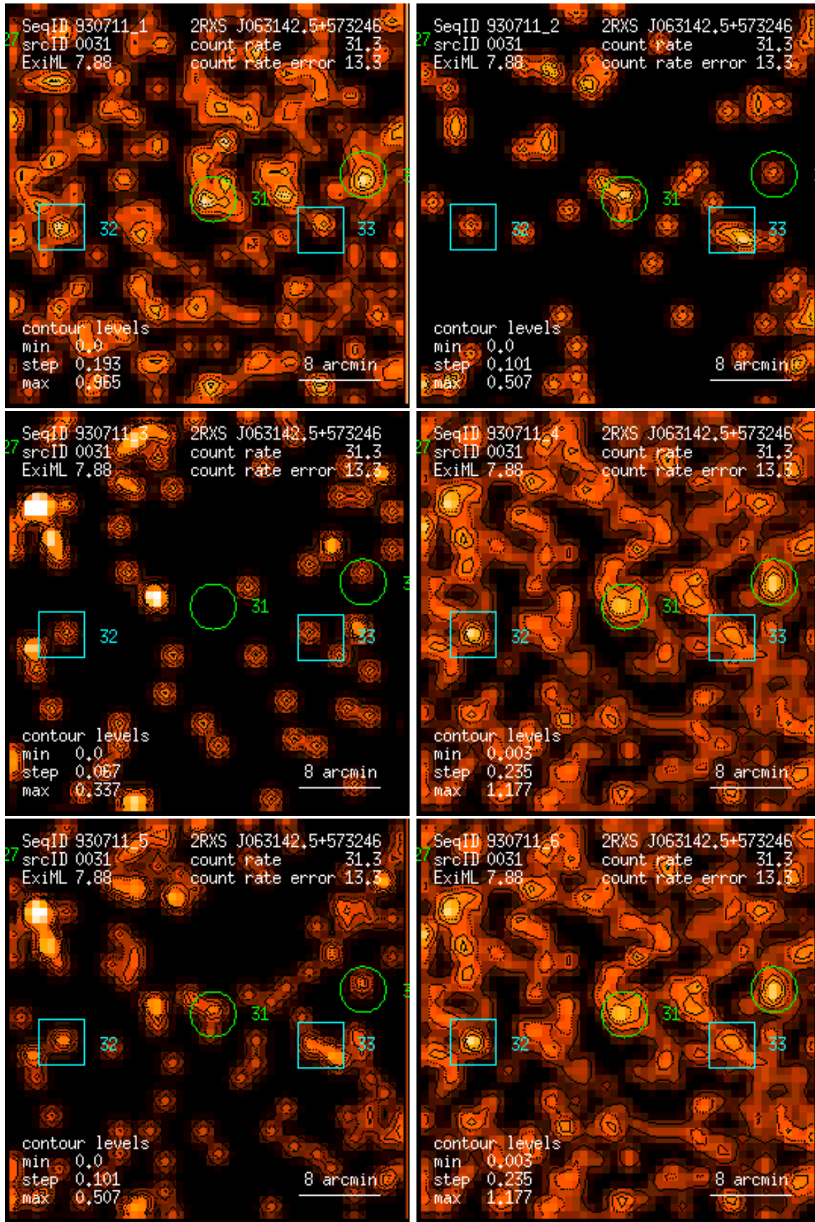
Figure 31: RASS 930711: detection 0031: band rate images, Gaussian filter: (1) PSPC channels 11 – 41, (2) 52 – 90, (3) 91 – 201, (4) 11 – 235, (5) 52 – 201, (6) 11 – 201. Broad band rates in counts/ks. Band rate contour levels in counts/ks/arcmin 2 .
