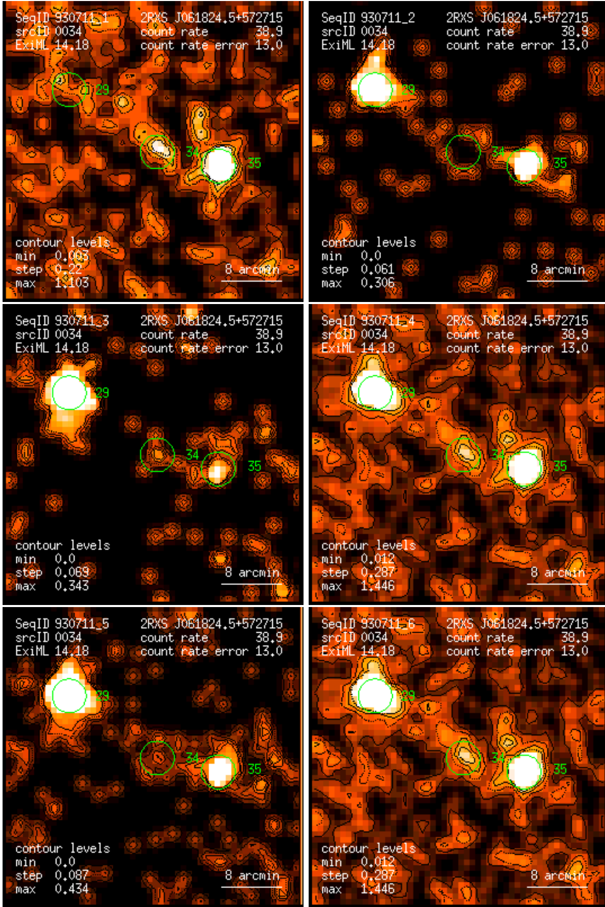
Figure 34: RASS 930711: detection 0034: band rate images, Gaussian filter: (1) PSPC channels 11 – 41, (2) 52 – 90, (3) 91 – 201, (4) 11 – 235, (5) 52 – 201, (6) 11 – 201. Broad band rates in counts/ks. Band rate contour levels in counts/ks/arcmin 2 .
