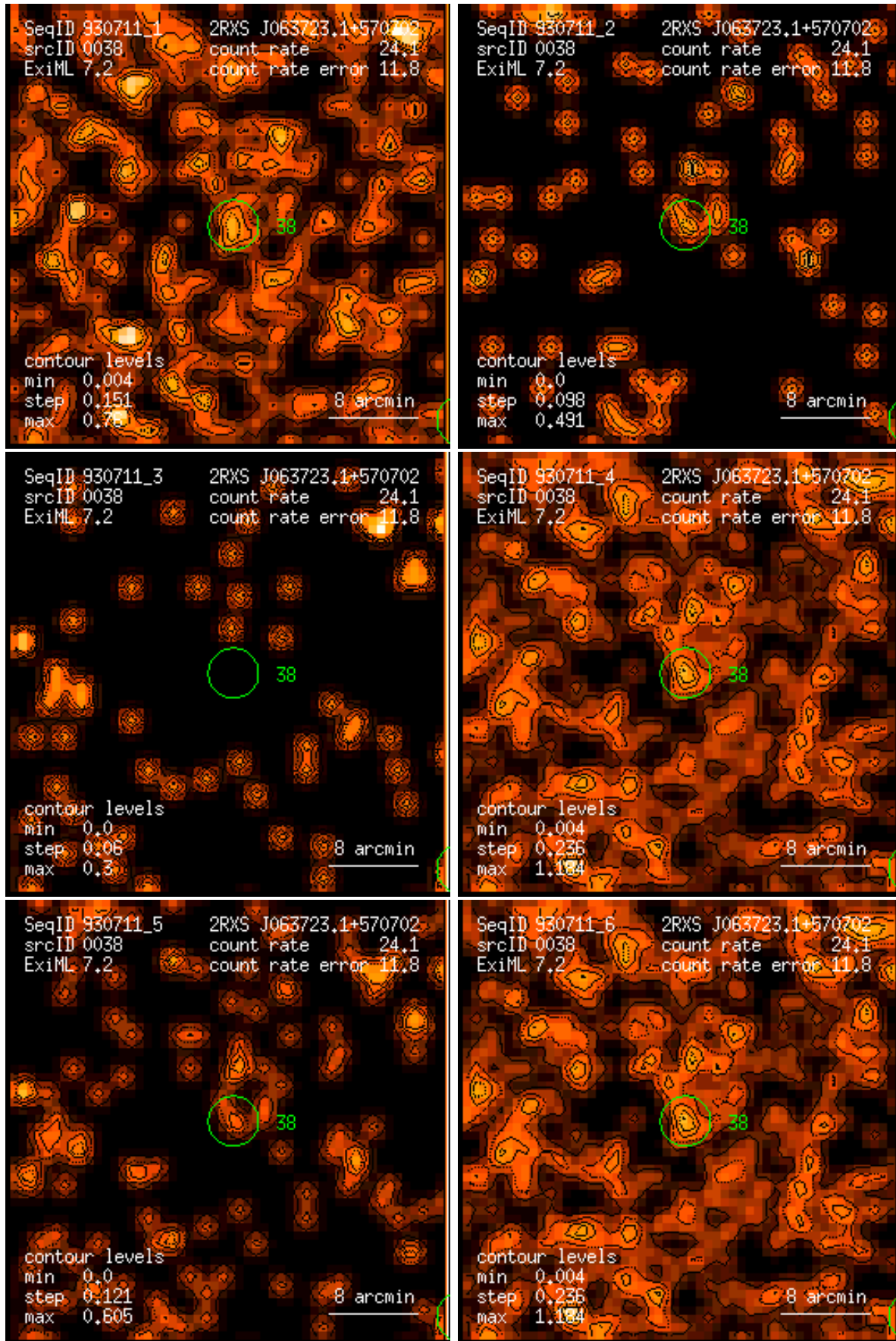
Figure 38: RASS 930711: detection 0038: band rate images, Gaussian filter: (1) PSPC channels 11 – 41, (2) 52 – 90, (3) 91 – 201, (4) 11 – 235, (5) 52 – 201, (6) 11 – 201. Broad band rates in counts/ks. Band rate contour levels in counts/ks/arcmin 2 .
