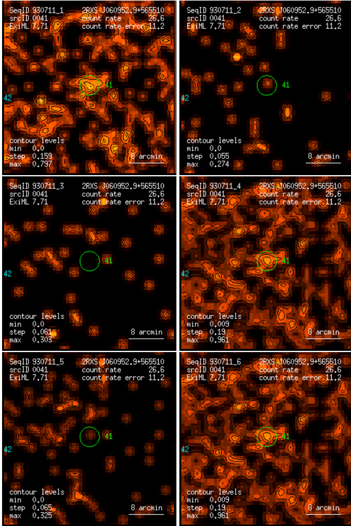
Figure 41: RASS 930711: detection 0041: band rate images, Gaussian filter: (1) PSPC channels 11 – 41, (2) 52 – 90, (3) 91 – 201, (4) 11 – 235, (5) 52 – 201, (6) 11 – 201. Broad band rates in counts/ks. Band rate contour levels in counts/ks/arcmin 2 .
