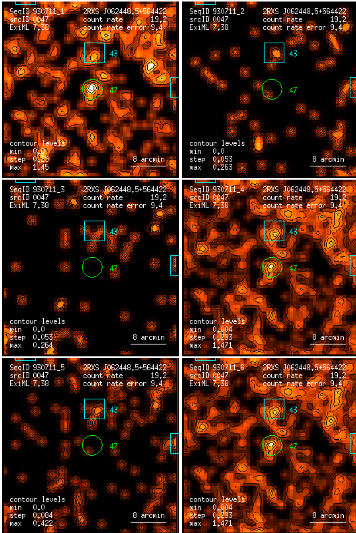
Figure 47: RASS 930711: detection 0047: band rate images, Gaussian filter: (1) PSPC channels 11 – 41, (2) 52 – 90, (3) 91 – 201, (4) 11 – 235, (5) 52 – 201, (6) 11 – 201. Broad band rates in counts/ks. Band rate contour levels in counts/ks/arcmin 2 .
