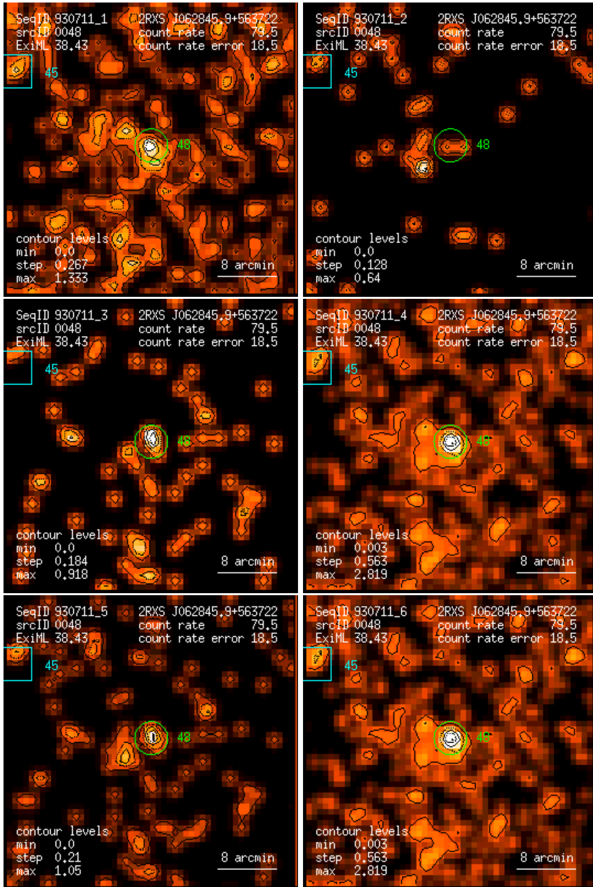
Figure 48: RASS 930711: detection 0048: band rate images, Gaussian filter: (1) PSPC channels 11 – 41, (2) 52 – 90, (3) 91 – 201, (4) 11 – 235, (5) 52 – 201, (6) 11 – 201. Broad band rates in counts/ks. Band rate contour levels in counts/ks/arcmin 2 .
