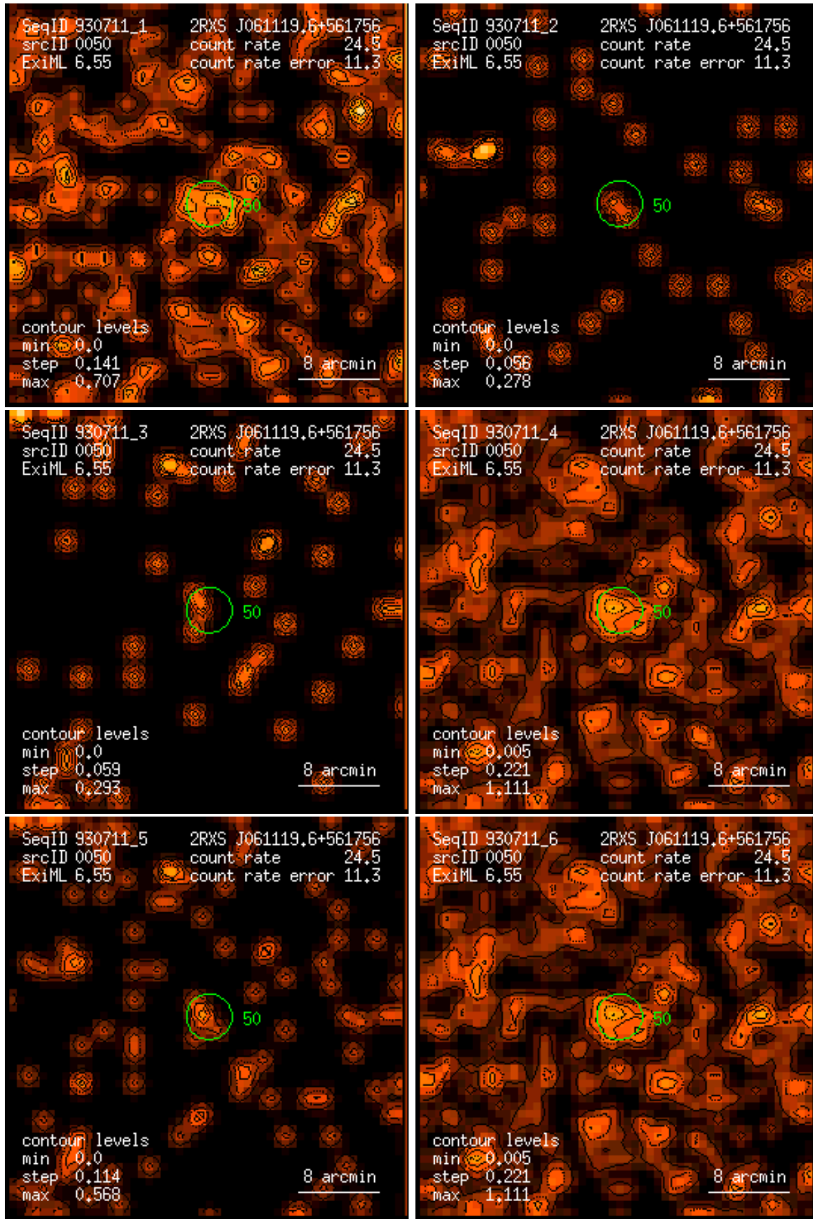
Figure 50: RASS 930711: detection 0050: band rate images, Gaussian filter: (1) PSPC channels 11 – 41, (2) 52 – 90, (3) 91 – 201, (4) 11 – 235, (5) 52 – 201, (6) 11 – 201. Broad band rates in counts/ks. Band rate contour levels in counts/ks/arcmin 2 .
