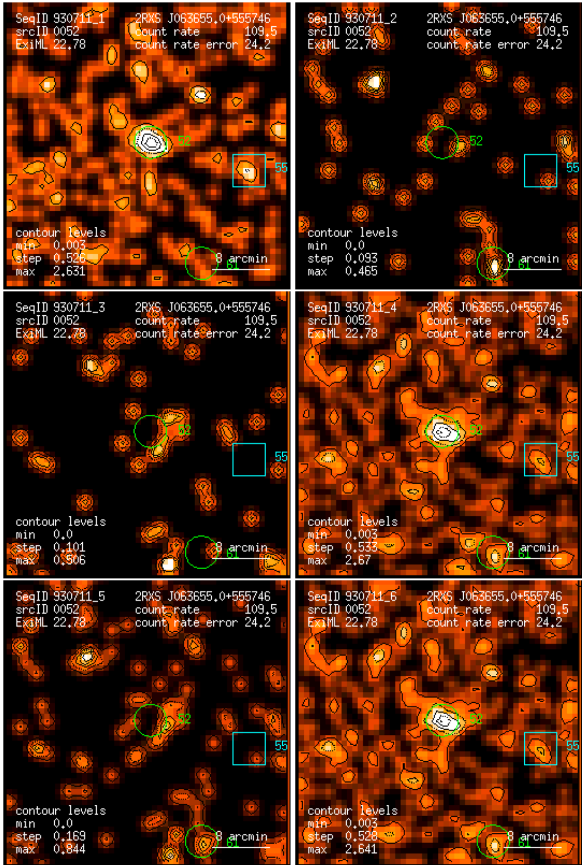
Figure 52: RASS 930711: detection 0052: band rate images, Gaussian filter: (1) PSPC channels 11 – 41, (2) 52 – 90, (3) 91 – 201, (4) 11 – 235, (5) 52 – 201, (6) 11 – 201. Broad band rates in counts/ks. Band rate contour levels in counts/ks/arcmin 2 .
