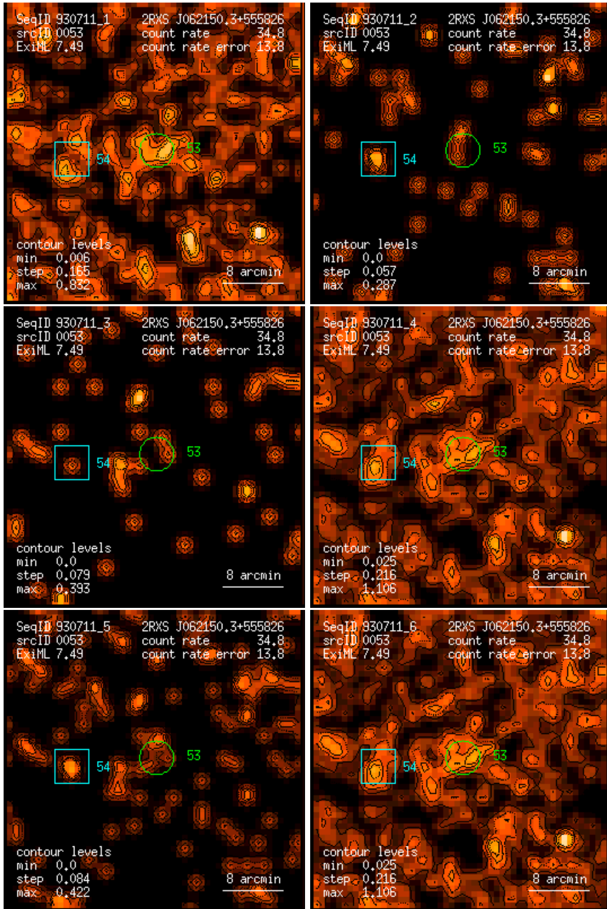
Figure 53: RASS 930711: detection 0053: band rate images, Gaussian filter: (1) PSPC channels 11 – 41, (2) 52 – 90, (3) 91 – 201, (4) 11 – 235, (5) 52 – 201, (6) 11 – 201. Broad band rates in counts/ks. Band rate contour levels in counts/ks/arcmin 2 .
