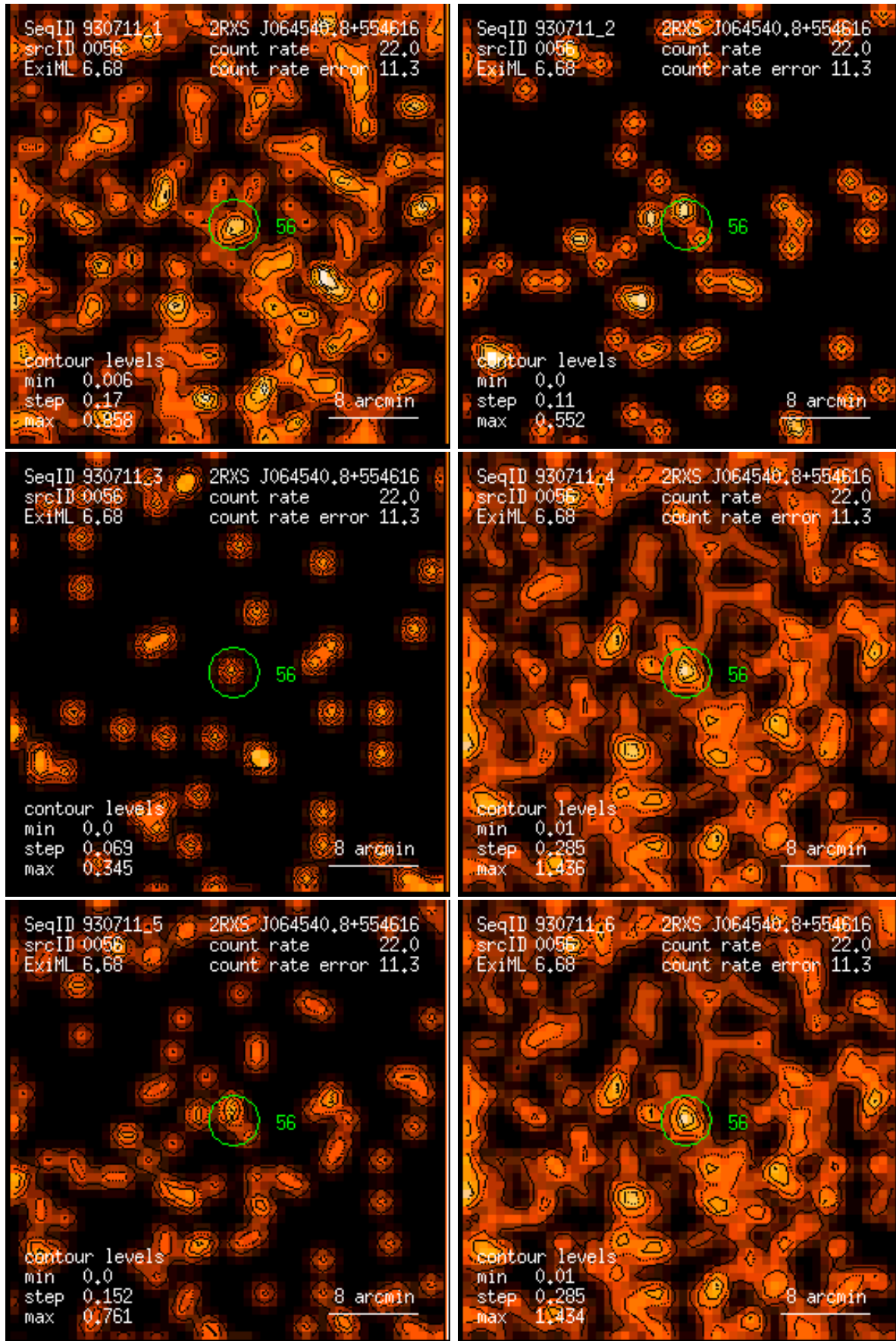
Figure 56: RASS 930711: detection 0056: band rate images, Gaussian filter: (1) PSPC channels 11 – 41, (2) 52 – 90, (3) 91 – 201, (4) 11 – 235, (5) 52 – 201, (6) 11 – 201. Broad band rates in counts/ks. Band rate contour levels in counts/ks/arcmin 2 .
