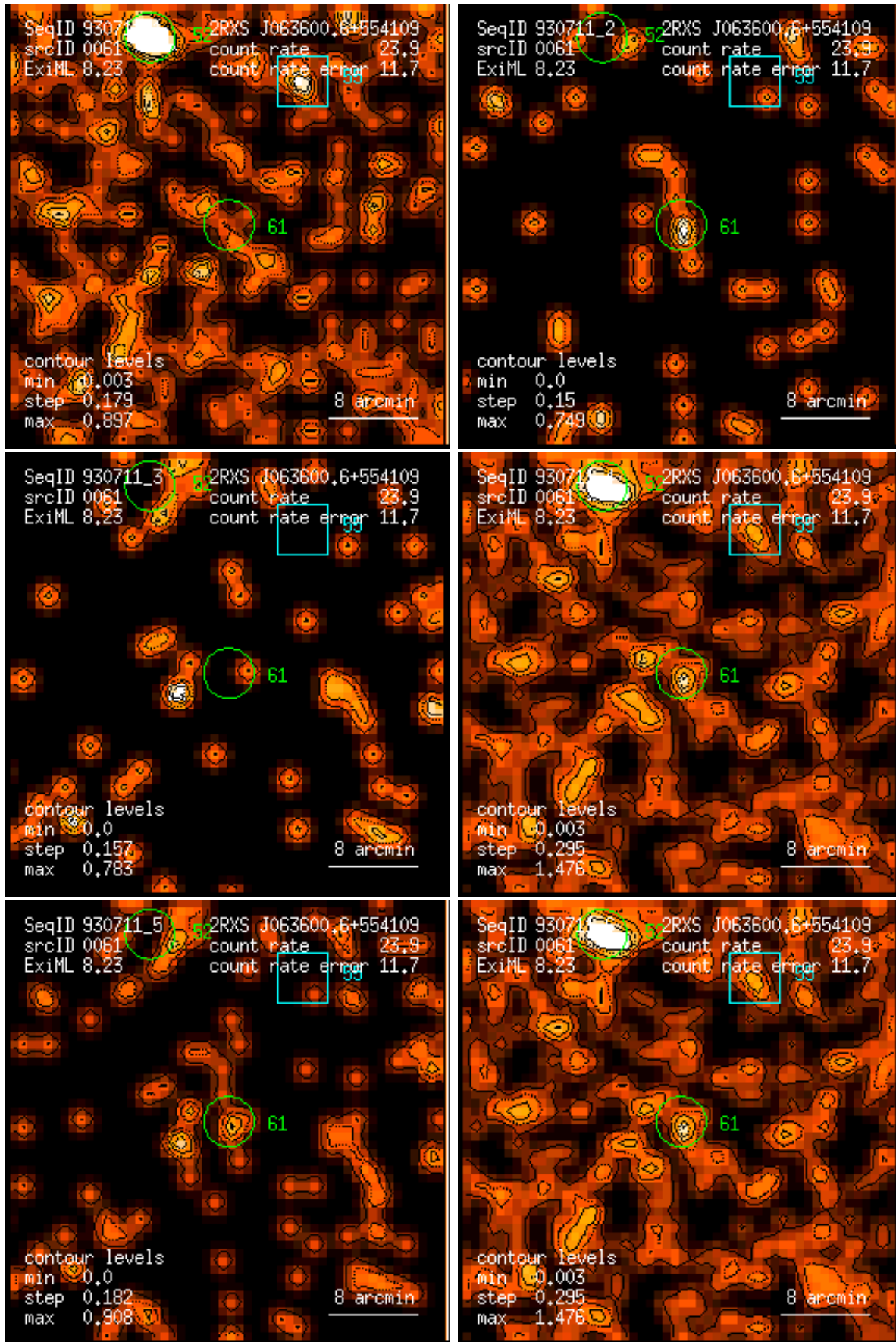
Figure 61: RASS 930711: detection 0061: band rate images, Gaussian filter: (1) PSPC channels 11 – 41, (2) 52 – 90, (3) 91 – 201, (4) 11 – 235, (5) 52 – 201, (6) 11 – 201. Broad band rates in counts/ks. Band rate contour levels in counts/ks/arcmin 2 .
