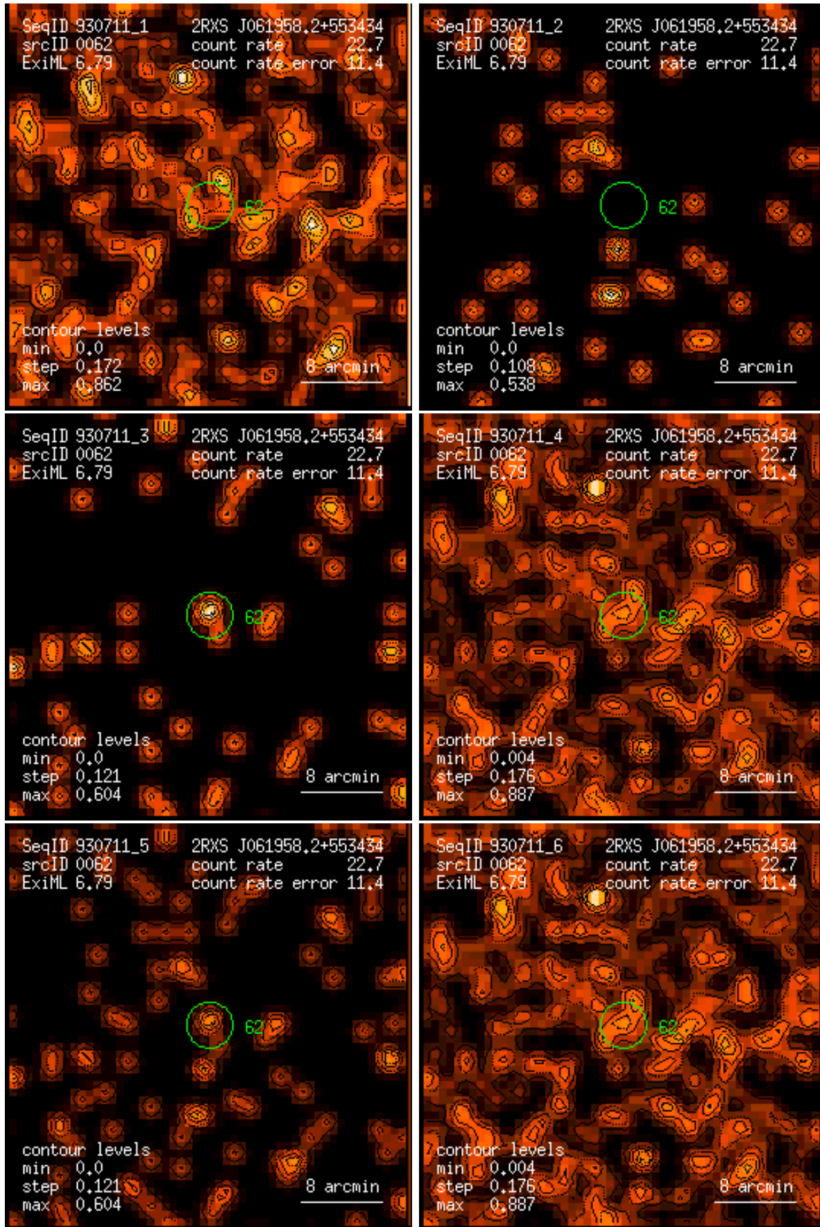
Figure 62: RASS 930711: detection 0062: band rate images, Gaussian filter: (1) PSPC channels 11 – 41, (2) 52 – 90, (3) 91 – 201, (4) 11 – 235, (5) 52 – 201, (6) 11 – 201. Broad band rates in counts/ks. Band rate contour levels in counts/ks/arcmin 2 .
