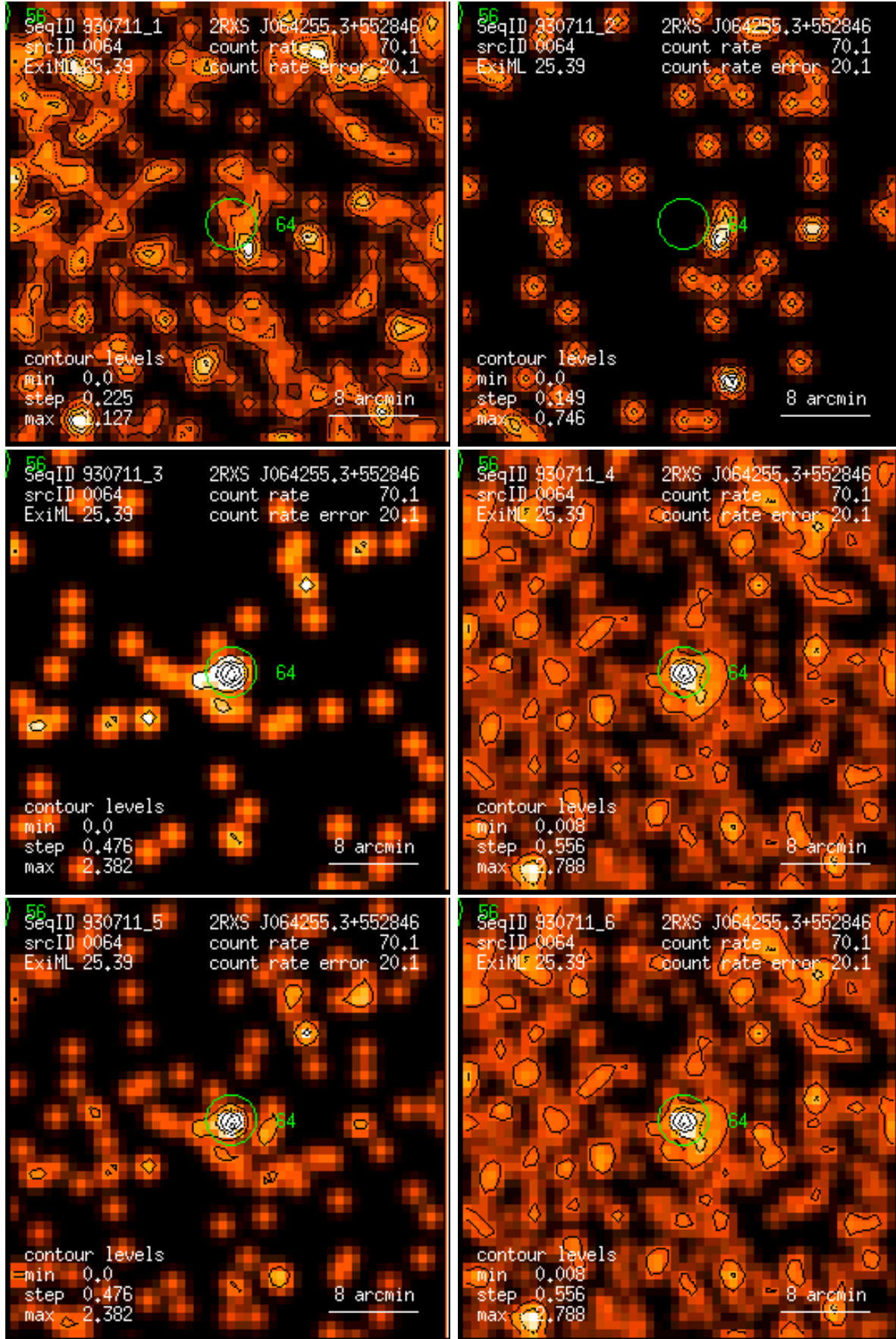
Figure 64: RASS 930711: detection 0064: band rate images, Gaussian filter: (1) PSPC channels 11 – 41, (2) 52 – 90, (3) 91 – 201, (4) 11 – 235, (5) 52 – 201, (6) 11 – 201. Broad band rates in counts/ks. Band rate contour levels in counts/ks/arcmin 2 .
