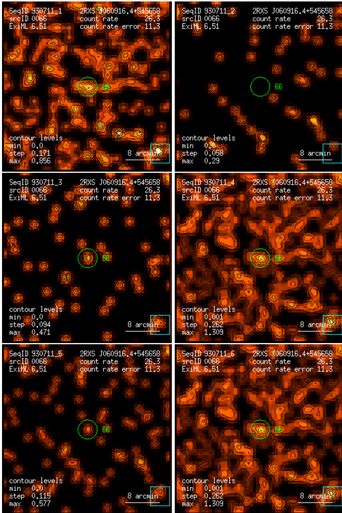
Figure 66: RASS 930711: detection 0066: band rate images, Gaussian filter: (1) PSPC channels 11 – 41, (2) 52 – 90, (3) 91 – 201, (4) 11 – 235, (5) 52 – 201, (6) 11 – 201. Broad band rates in counts/ks. Band rate contour levels in counts/ks/arcmin 2 .
