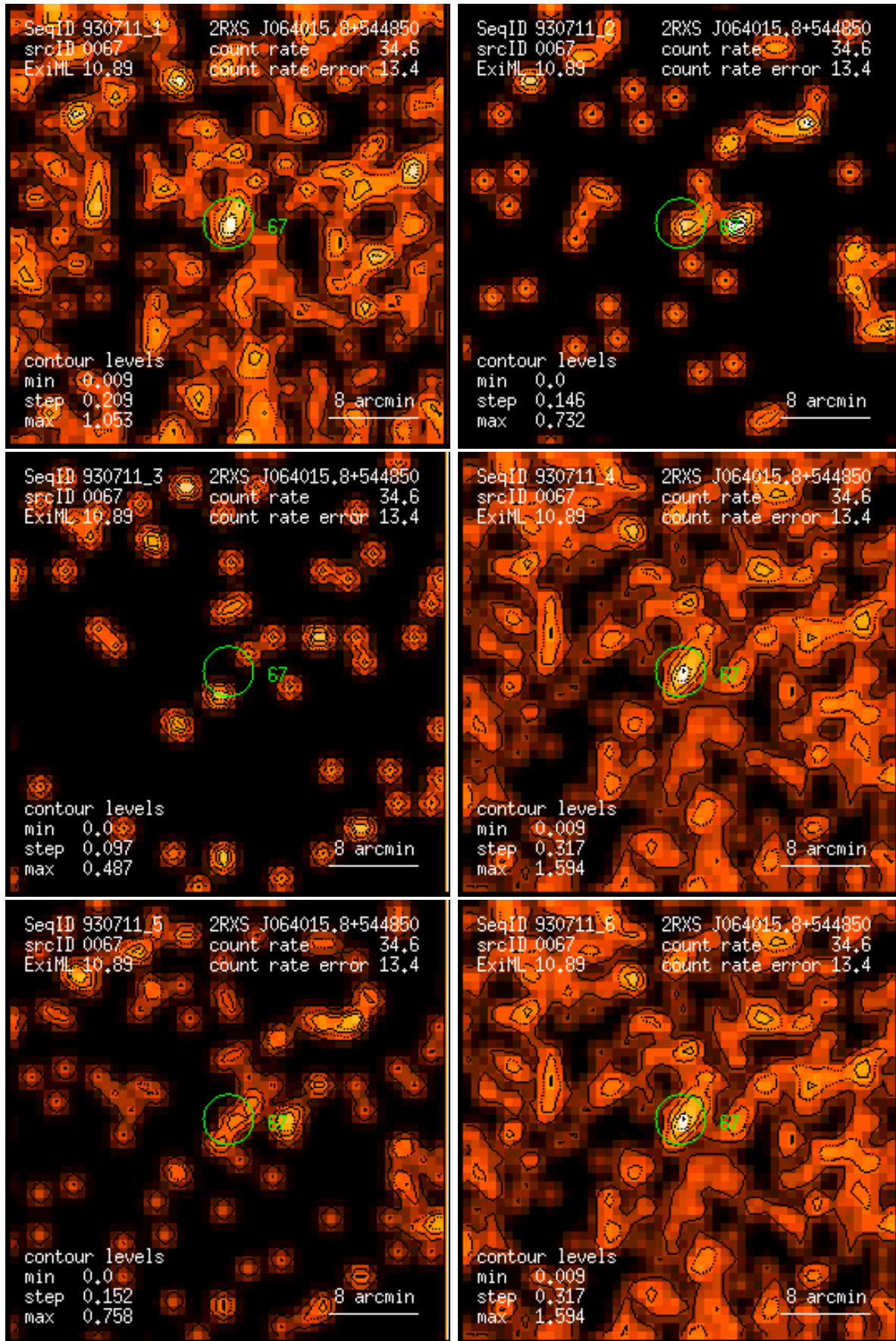
Figure 67: RASS 930711: detection 0067: band rate images, Gaussian filter: (1) PSPC channels 11 – 41, (2) 52 – 90, (3) 91 – 201, (4) 11 – 235, (5) 52 – 201, (6) 11 – 201. Broad band rates in counts/ks. Band rate contour levels in counts/ks/arcmin 2 .
