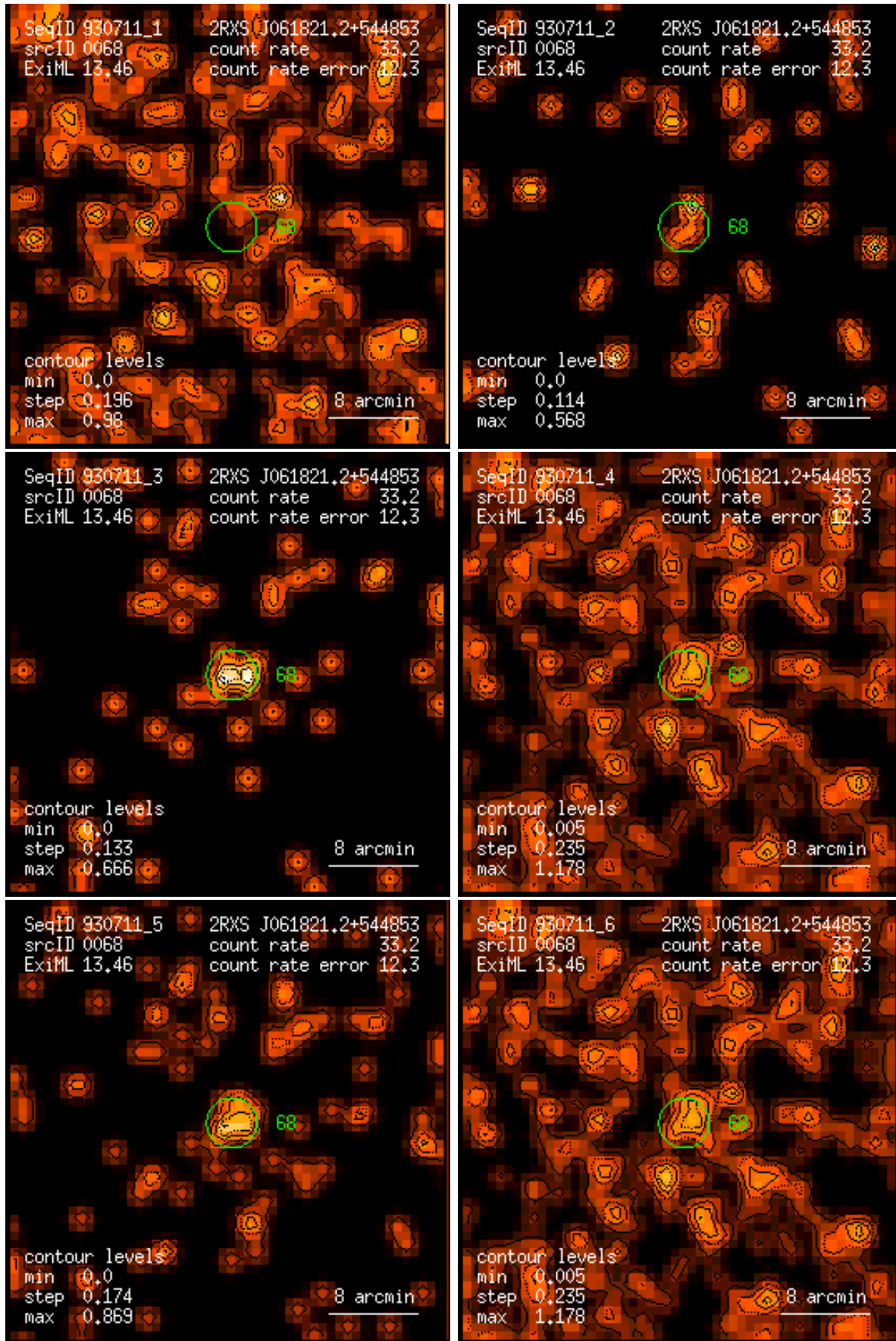
Figure 68: RASS 930711: detection 0068: band rate images, Gaussian filter: (1) PSPC channels 11 – 41, (2) 52 – 90, (3) 91 – 201, (4) 11 – 235, (5) 52 – 201, (6) 11 – 201. Broad band rates in counts/ks. Band rate contour levels in counts/ks/arcmin 2 .
