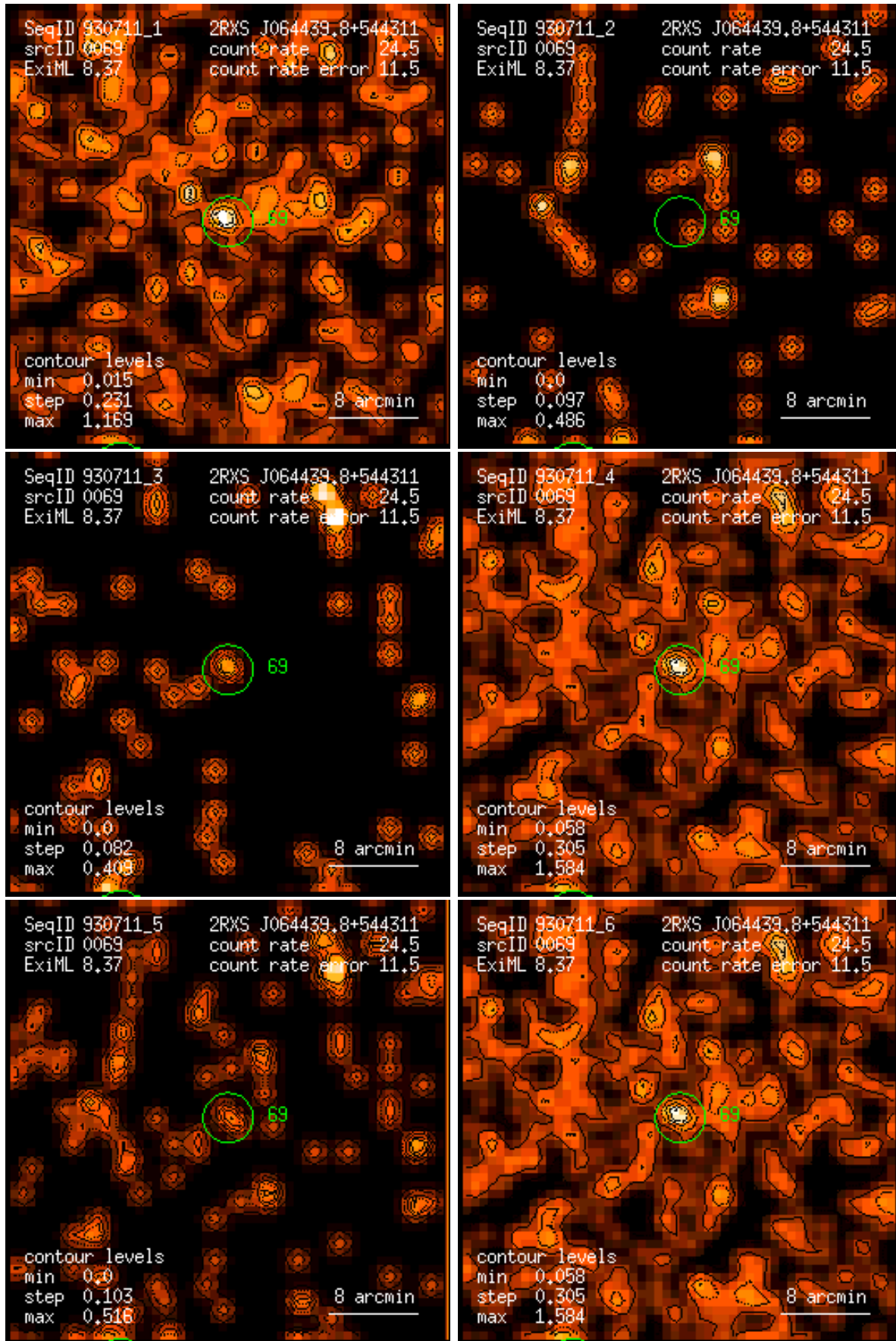
Figure 69: RASS 930711: detection 0069: band rate images, Gaussian filter: (1) PSPC channels 11 – 41, (2) 52 – 90, (3) 91 – 201, (4) 11 – 235, (5) 52 – 201, (6) 11 – 201. Broad band rates in counts/ks. Band rate contour levels in counts/ks/arcmin 2 .
