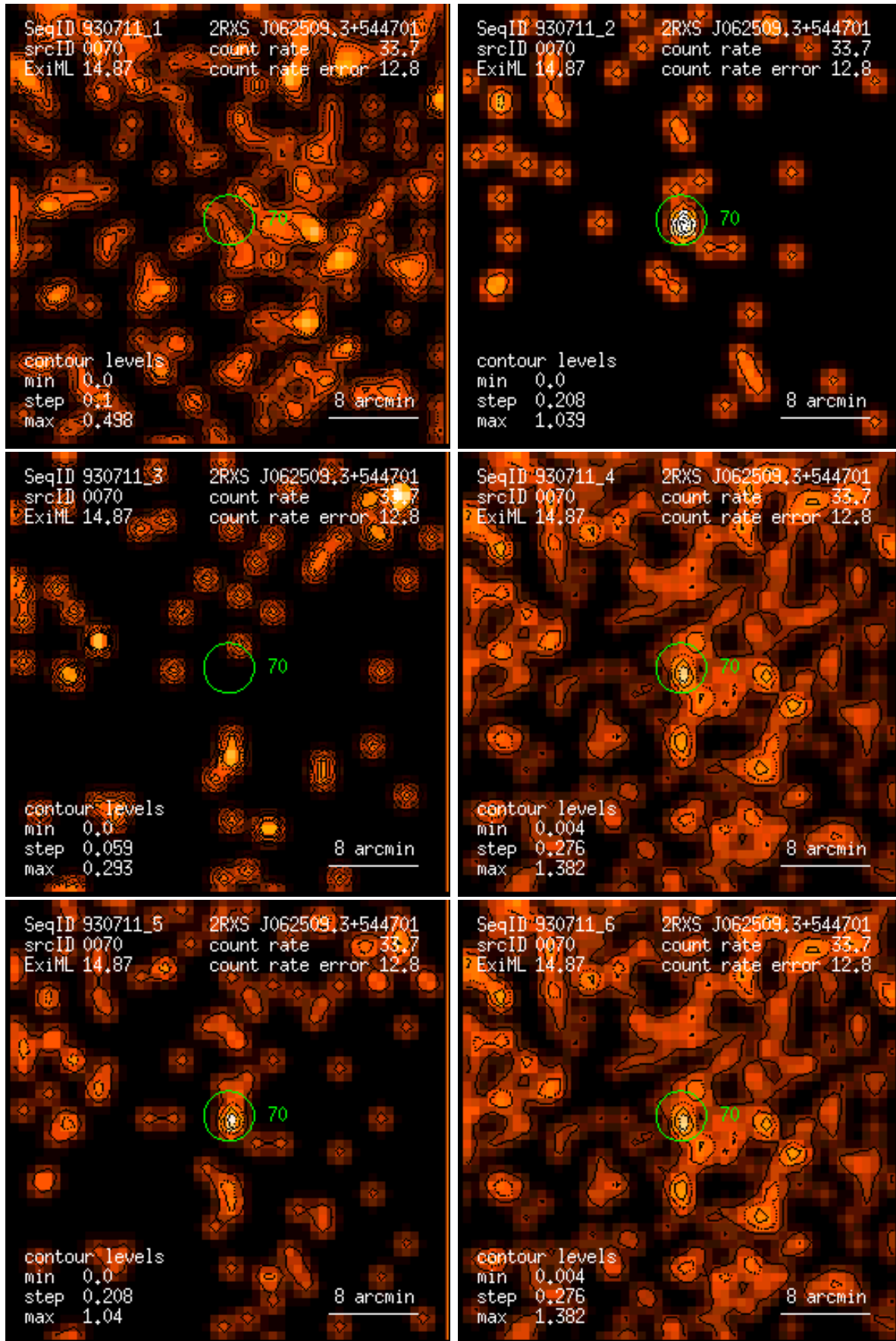
Figure 70: RASS 930711: detection 0070: band rate images, Gaussian filter: (1) PSPC channels 11 – 41, (2) 52 – 90, (3) 91 – 201, (4) 11 – 235, (5) 52 – 201, (6) 11 – 201. Broad band rates in counts/ks. Band rate contour levels in counts/ks/arcmin 2 .
