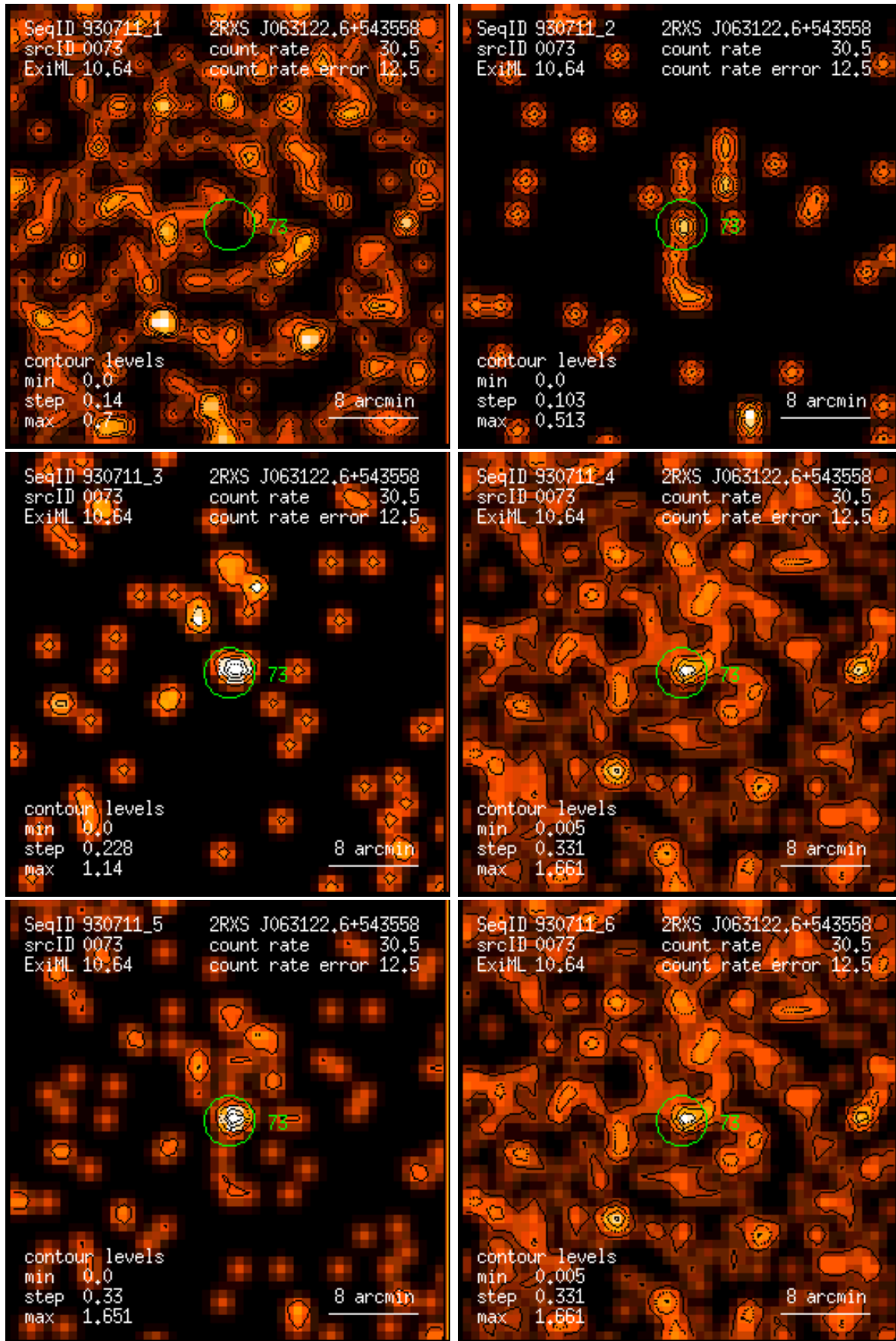
Figure 73: RASS 930711: detection 0073: band rate images, Gaussian filter: (1) PSPC channels 11 – 41, (2) 52 – 90, (3) 91 – 201, (4) 11 – 235, (5) 52 – 201, (6) 11 – 201. Broad band rates in counts/ks. Band rate contour levels in counts/ks/arcmin 2 .
