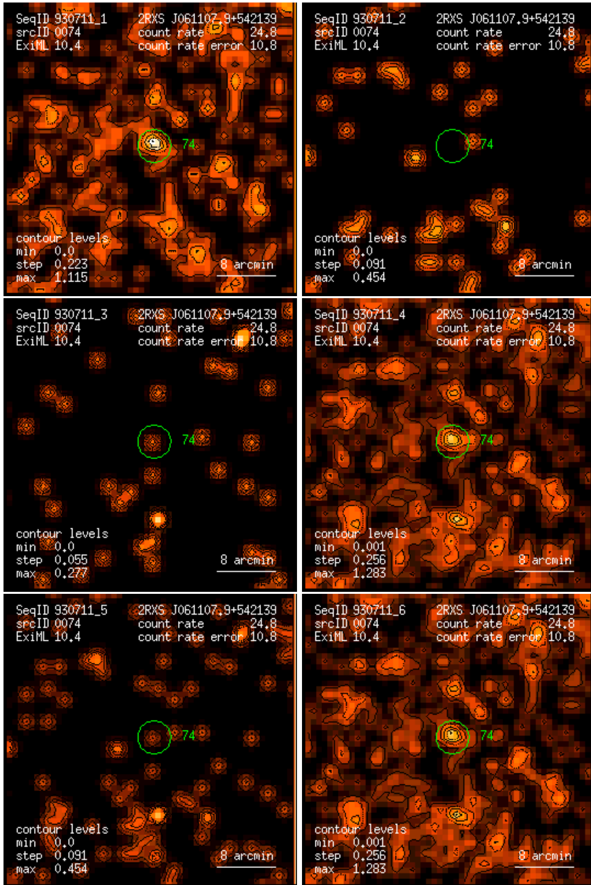
Figure 74: RASS 930711: detection 0074: band rate images, Gaussian filter: (1) PSPC channels 11 – 41, (2) 52 – 90, (3) 91 – 201, (4) 11 – 235, (5) 52 – 201, (6) 11 – 201. Broad band rates in counts/ks. Band rate contour levels in counts/ks/arcmin 2 .
