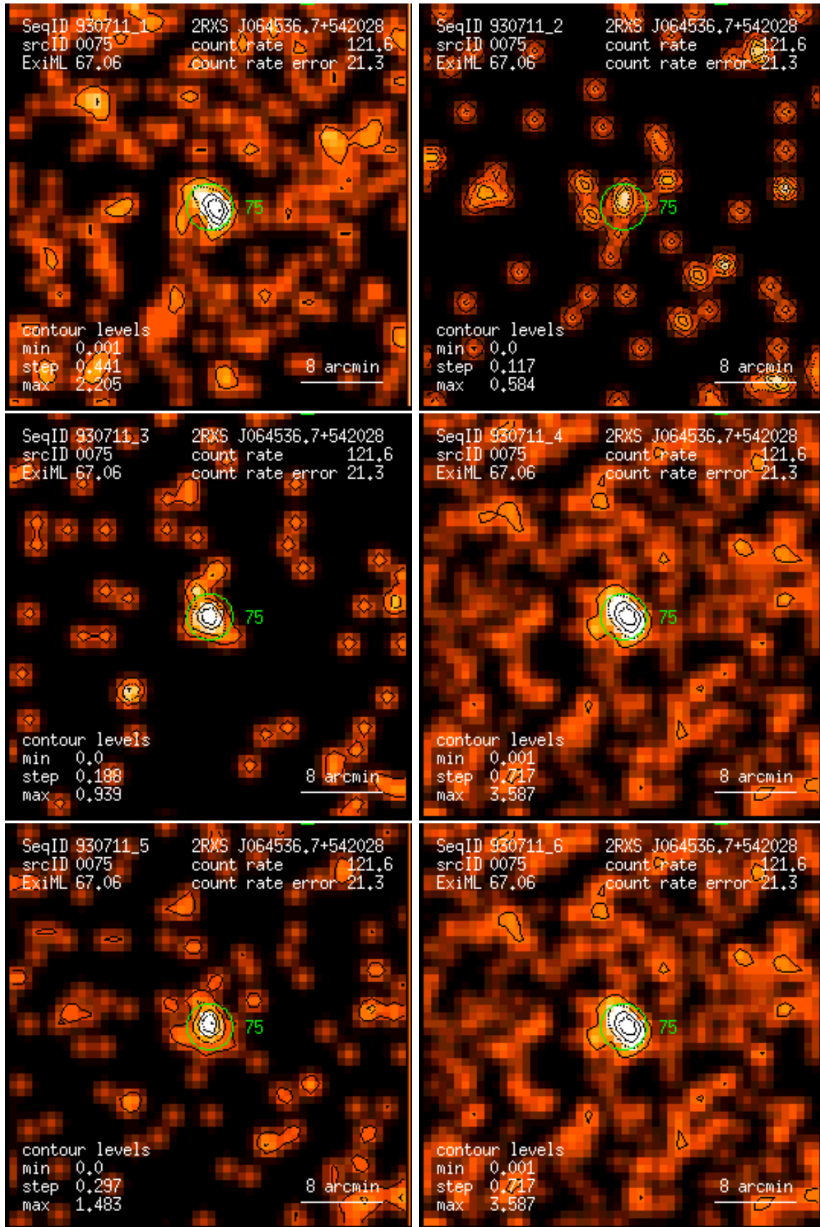
Figure 75: RASS 930711: detection 0075: band rate images, Gaussian filter: (1) PSPC channels 11 – 41, (2) 52 – 90, (3) 91 – 201, (4) 11 – 235, (5) 52 – 201, (6) 11 – 201. Broad band rates in counts/ks. Band rate contour levels in counts/ks/arcmin 2 .
