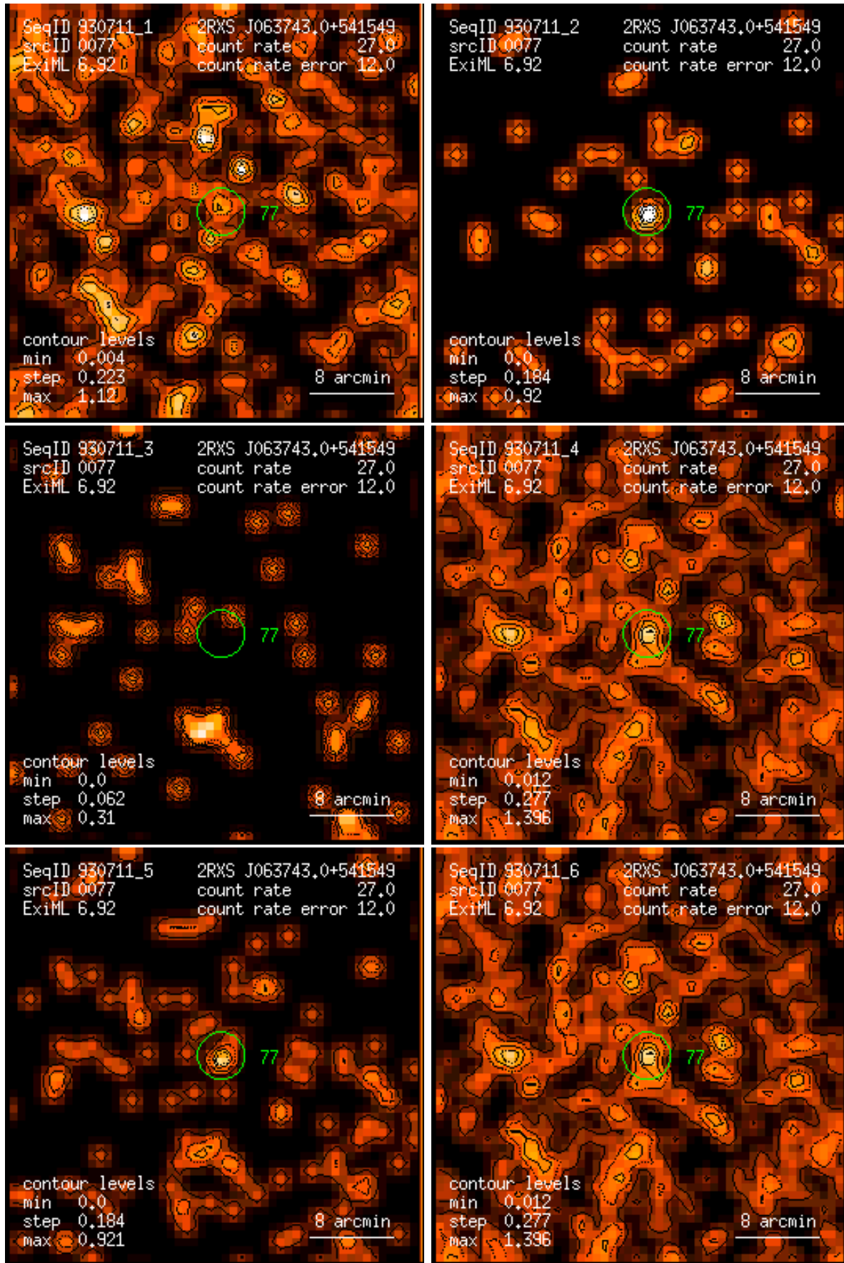
Figure 77: RASS 930711: detection 0077: band rate images, Gaussian filter: (1) PSPC channels 11 – 41, (2) 52 – 90, (3) 91 – 201, (4) 11 – 235, (5) 52 – 201, (6) 11 – 201. Broad band rates in counts/ks. Band rate contour levels in counts/ks/arcmin 2 .
