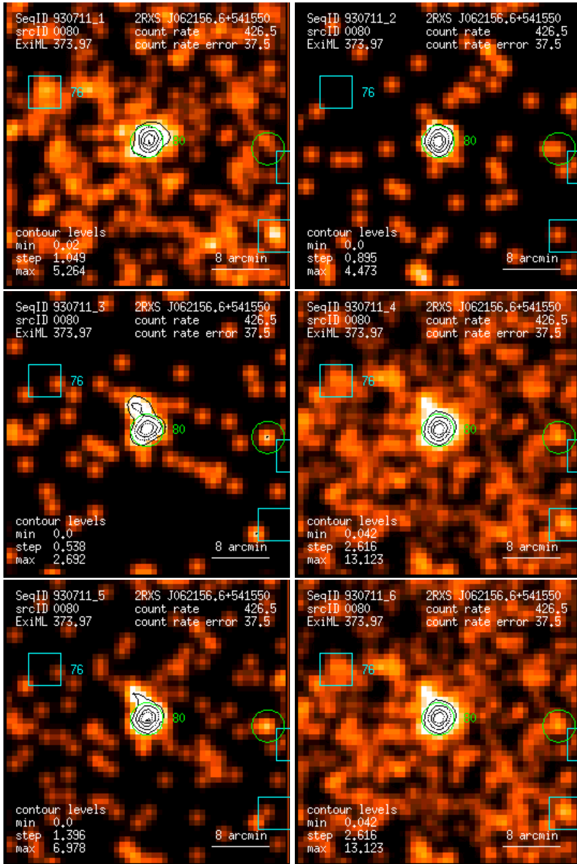
Figure 80: RASS 930711: detection 0080: band rate images, Gaussian filter: (1) PSPC channels 11 – 41, (2) 52 – 90, (3) 91 – 201, (4) 11 – 235, (5) 52 – 201, (6) 11 – 201. Broad band rates in counts/ks. Band rate contour levels in counts/ks/arcmin 2 .
