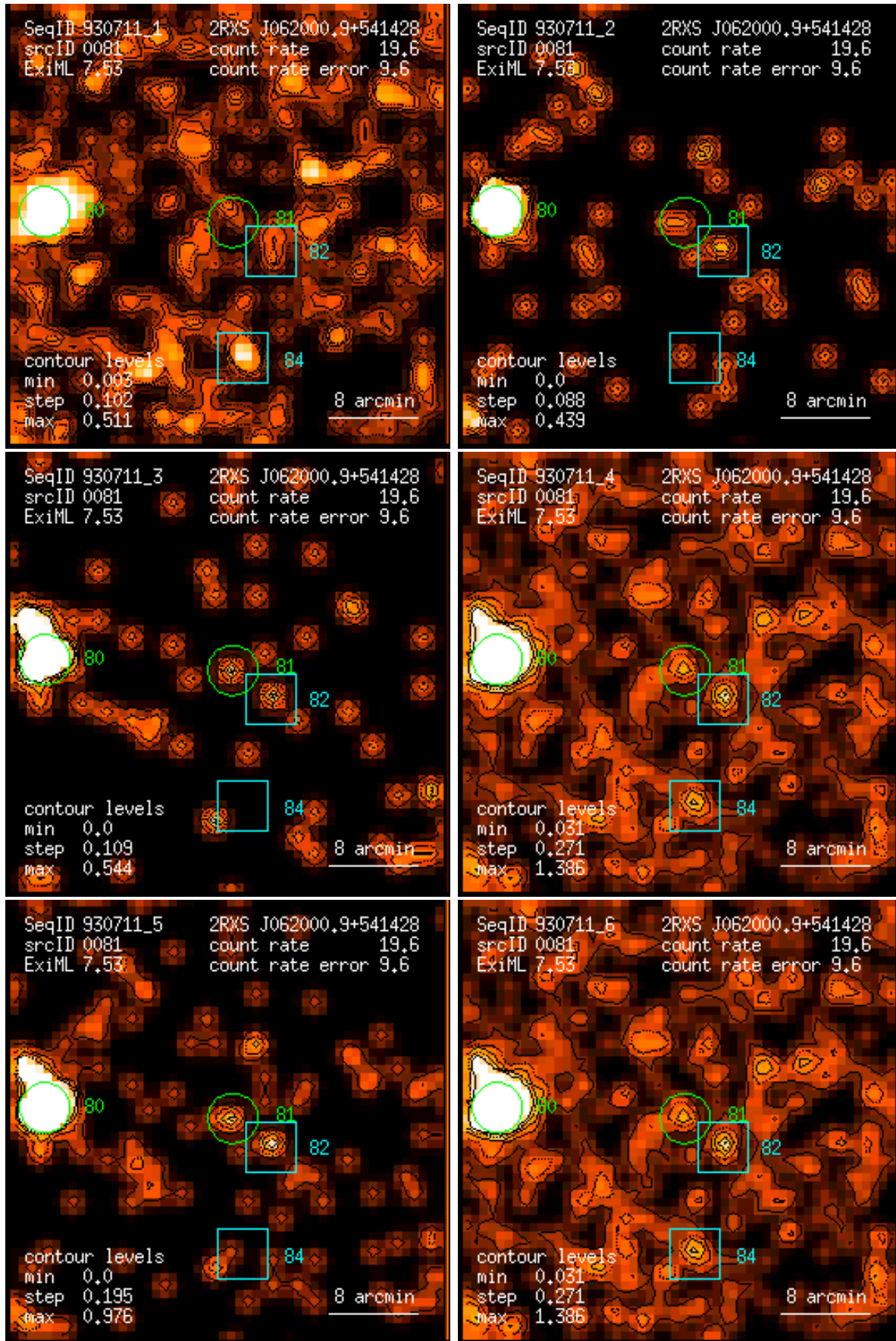
Figure 81: RASS 930711: detection 0081: band rate images, Gaussian filter: (1) PSPC channels 11 – 41, (2) 52 – 90, (3) 91 – 201, (4) 11 – 235, (5) 52 – 201, (6) 11 – 201. Broad band rates in counts/ks. Band rate contour levels in counts/ks/arcmin 2 .
