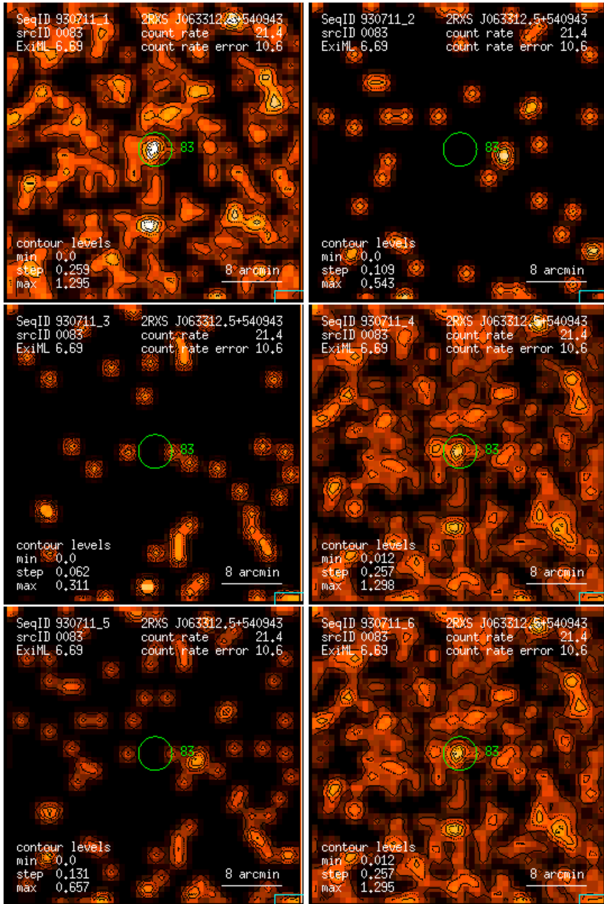
Figure 83: RASS 930711: detection 0083: band rate images, Gaussian filter: (1) PSPC channels 11 – 41, (2) 52 – 90, (3) 91 – 201, (4) 11 – 235, (5) 52 – 201, (6) 11 – 201. Broad band rates in counts/ks. Band rate contour levels in counts/ks/arcmin 2 .
