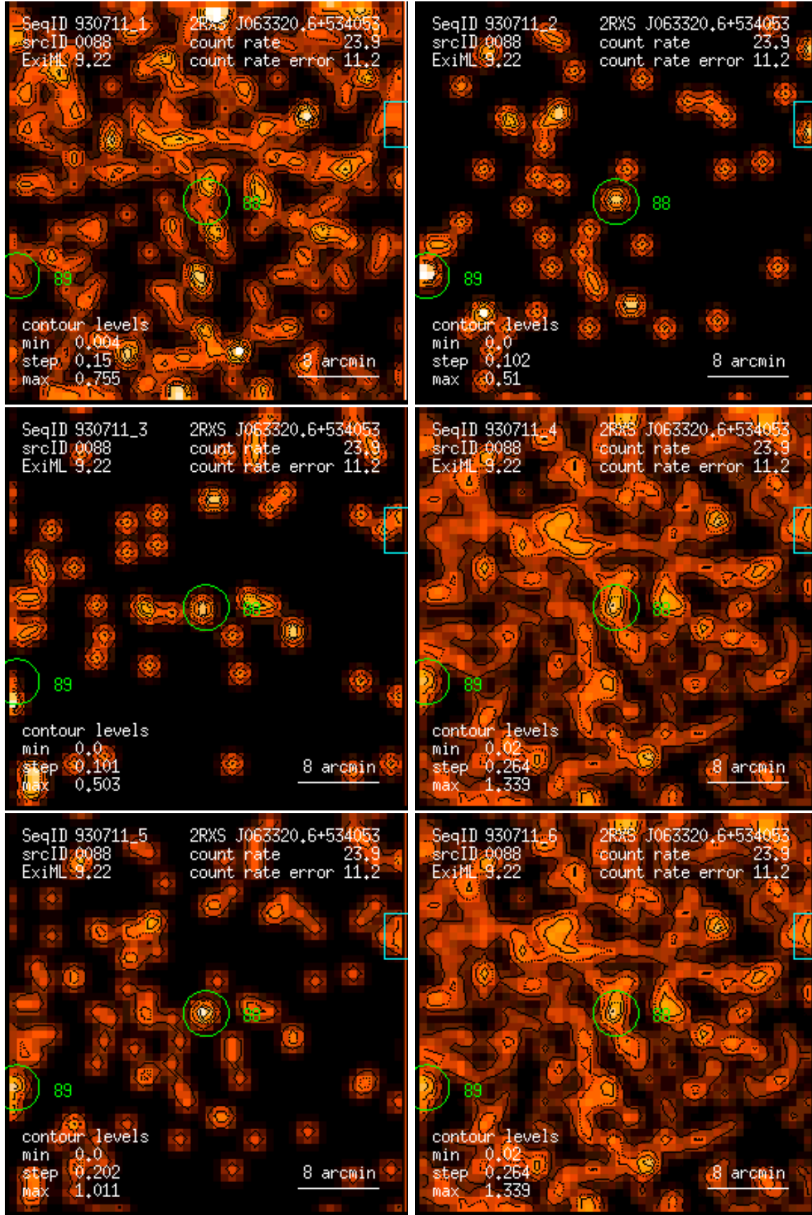
Figure 88: RASS 930711: detection 0088: band rate images, Gaussian filter: (1) PSPC channels 11 – 41, (2) 52 – 90, (3) 91 – 201, (4) 11 – 235, (5) 52 – 201, (6) 11 – 201. Broad band rates in counts/ks. Band rate contour levels in counts/ks/arcmin 2 .
