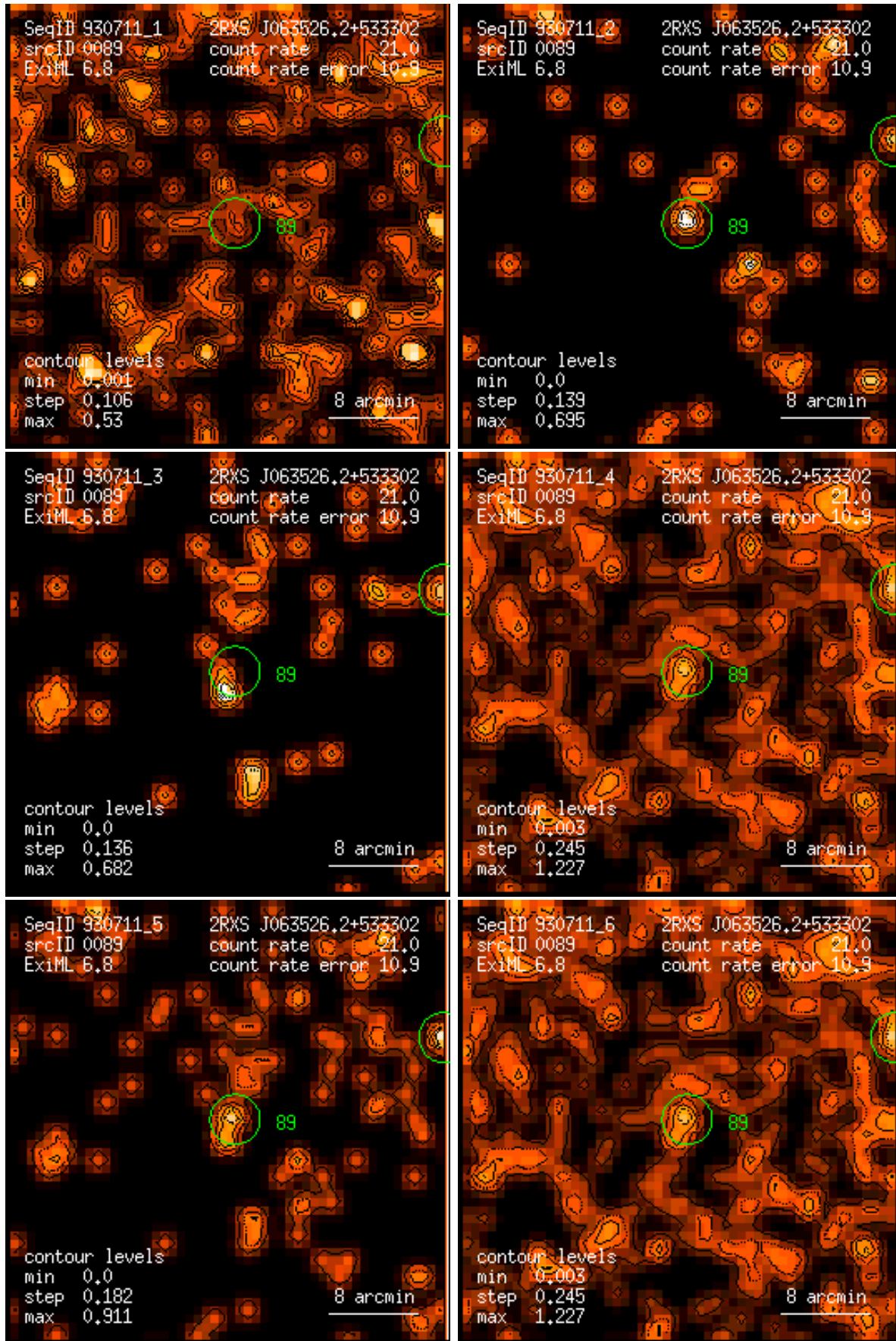
Figure 89: RASS 930711: detection 0089: band rate images, Gaussian filter: (1) PSPC channels 11 – 41, (2) 52 – 90, (3) 91 – 201, (4) 11 – 235, (5) 52 – 201, (6) 11 – 201. Broad band rates in counts/ks. Band rate contour levels in counts/ks/arcmin 2 .
