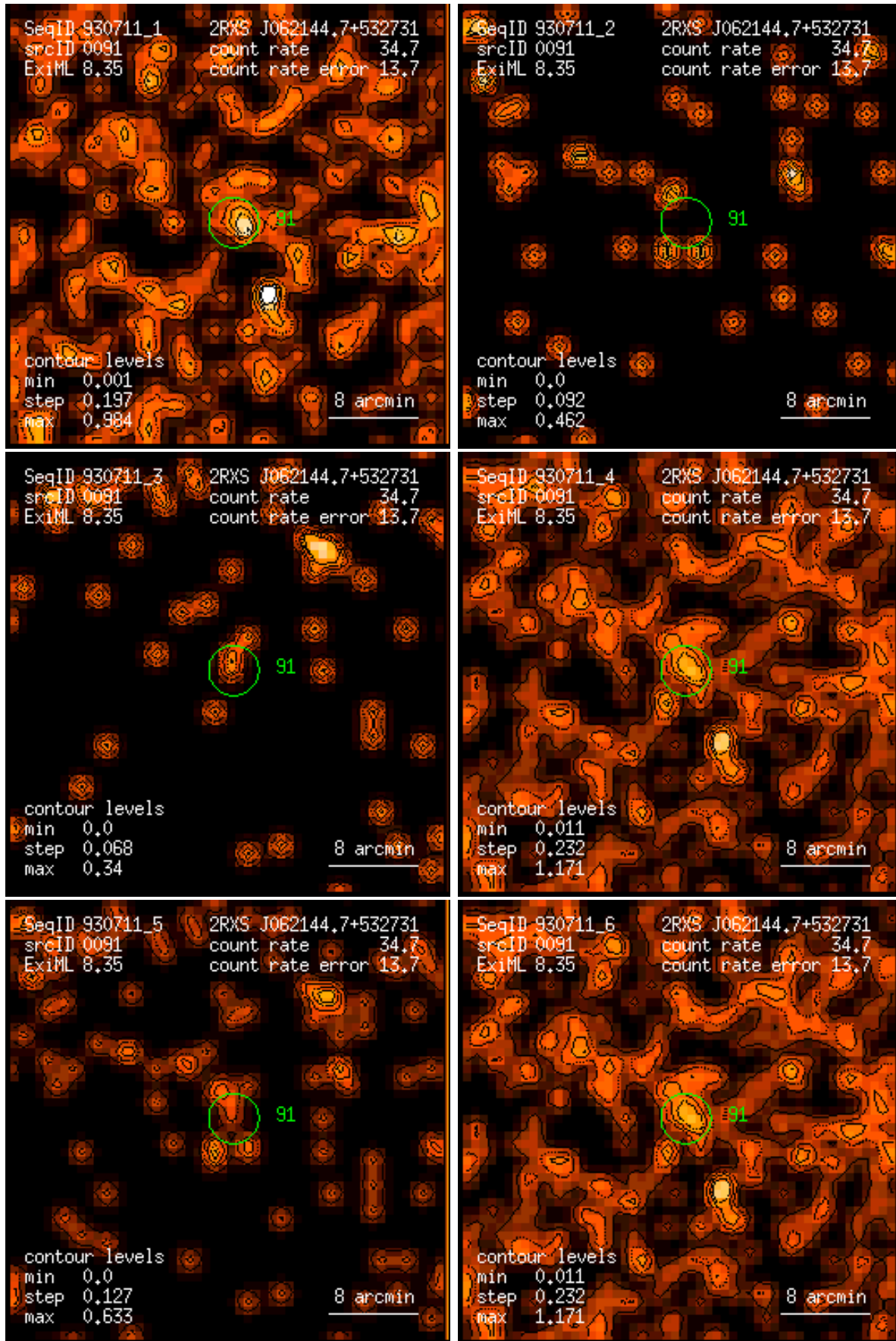
Figure 91: RASS 930711: detection 0091: band rate images, Gaussian filter: (1) PSPC channels 11 – 41, (2) 52 – 90, (3) 91 – 201, (4) 11 – 235, (5) 52 – 201, (6) 11 – 201. Broad band rates in counts/ks. Band rate contour levels in counts/ks/arcmin 2 .
