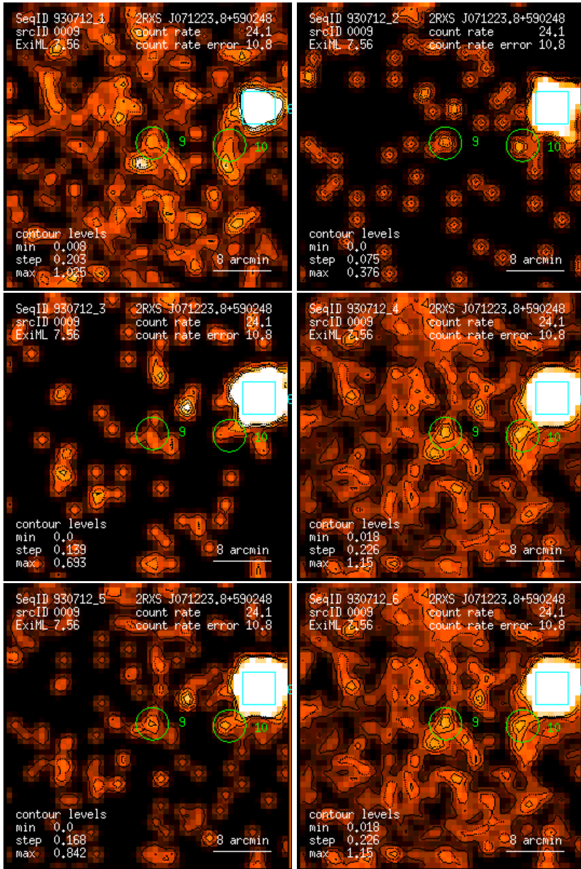
Figure 9: RASS 930712: detection 0009: band rate images, Gaussian filter: (1) PSPC channels 11 – 41, (2) 52 – 90, (3) 91 – 201, (4) 11 – 235, (5) 52 – 201, (6) 11 – 201. Broad band rates in counts/ks. Band rate contour levels in counts/ks/arcmin 2 .
