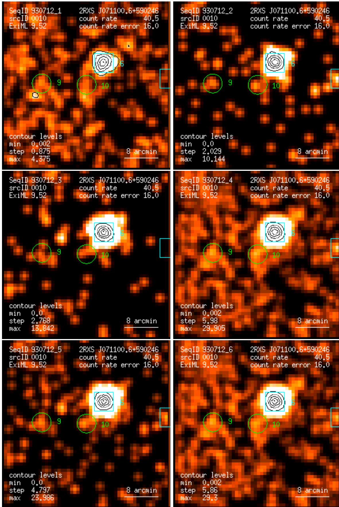
Figure 10: RASS 930712: detection 0010: band rate images, Gaussian filter: (1) PSPC channels 11 – 41, (2) 52 – 90, (3) 91 – 201, (4) 11 – 235, (5) 52 – 201, (6) 11 – 201. Broad band rates in counts/ks. Band rate contour levels in counts/ks/arcmin 2 .
