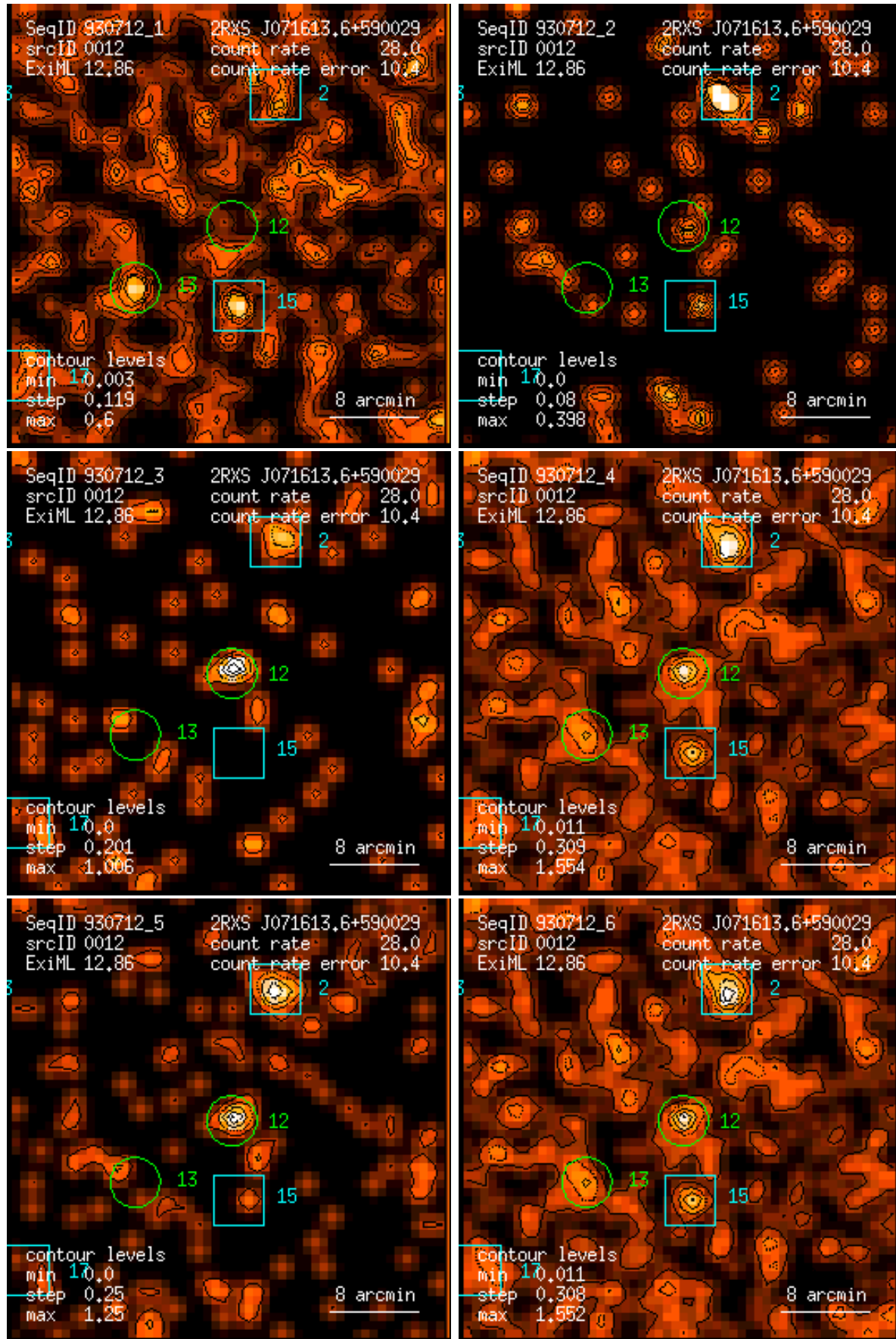
Figure 12: RASS 930712: detection 0012: band rate images, Gaussian filter: (1) PSPC channels 11 – 41, (2) 52 – 90, (3) 91 – 201, (4) 11 – 235, (5) 52 – 201, (6) 11 – 201. Broad band rates in counts/ks. Band rate contour levels in counts/ks/arcmin 2 .
