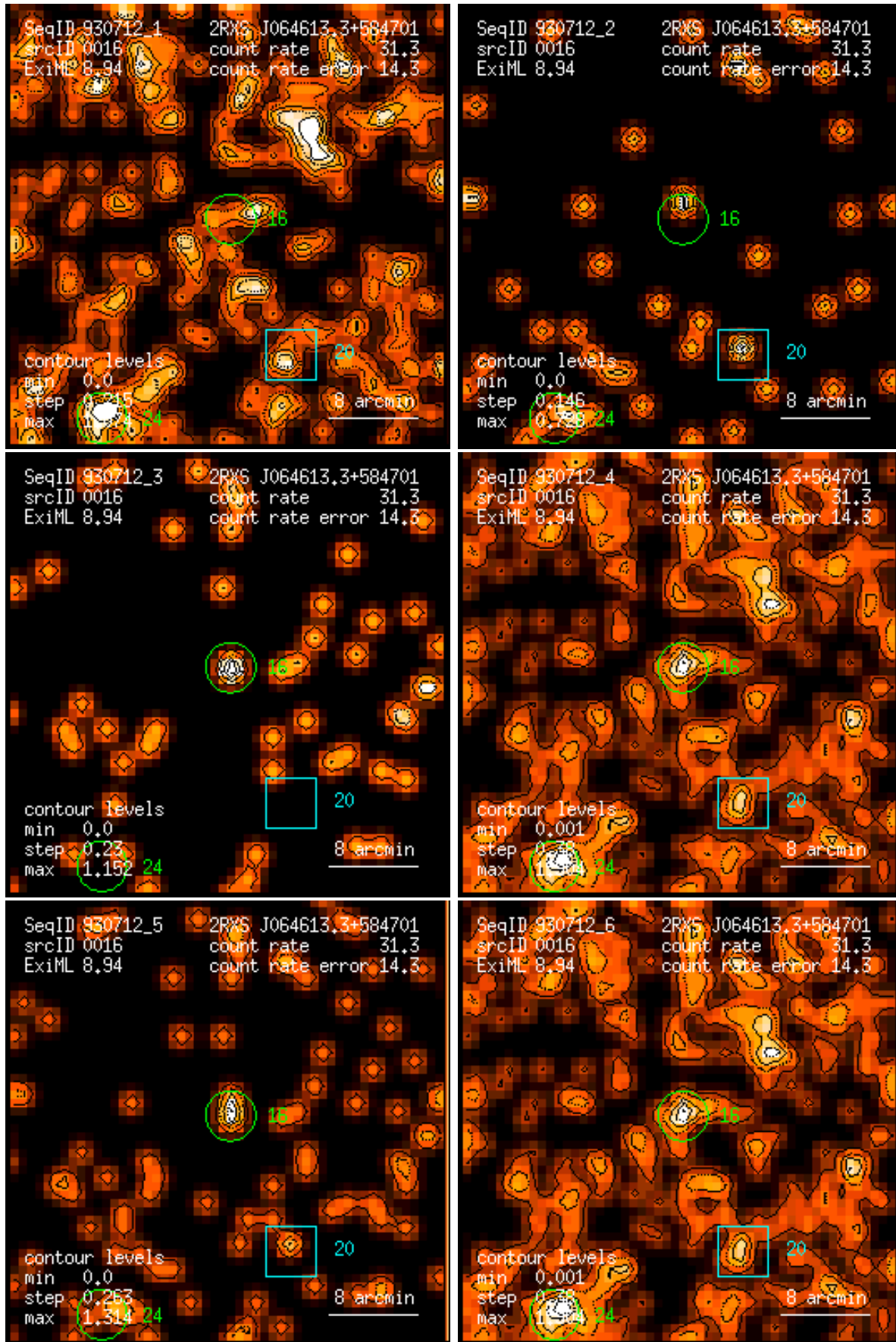
Figure 16: RASS 930712: detection 0016: band rate images, Gaussian filter: (1) PSPC channels 11 – 41, (2) 52 – 90, (3) 91 – 201, (4) 11 – 235, (5) 52 – 201, (6) 11 – 201. Broad band rates in counts/ks. Band rate contour levels in counts/ks/arcmin 2 .
