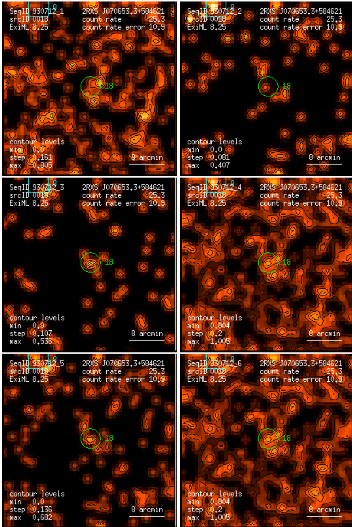
Figure 18: RASS 930712: detection 0018: band rate images, Gaussian filter: (1) PSPC channels 11 – 41, (2) 52 – 90, (3) 91 – 201, (4) 11 – 235, (5) 52 – 201, (6) 11 – 201. Broad band rates in counts/ks. Band rate contour levels in counts/ks/arcmin 2 .
