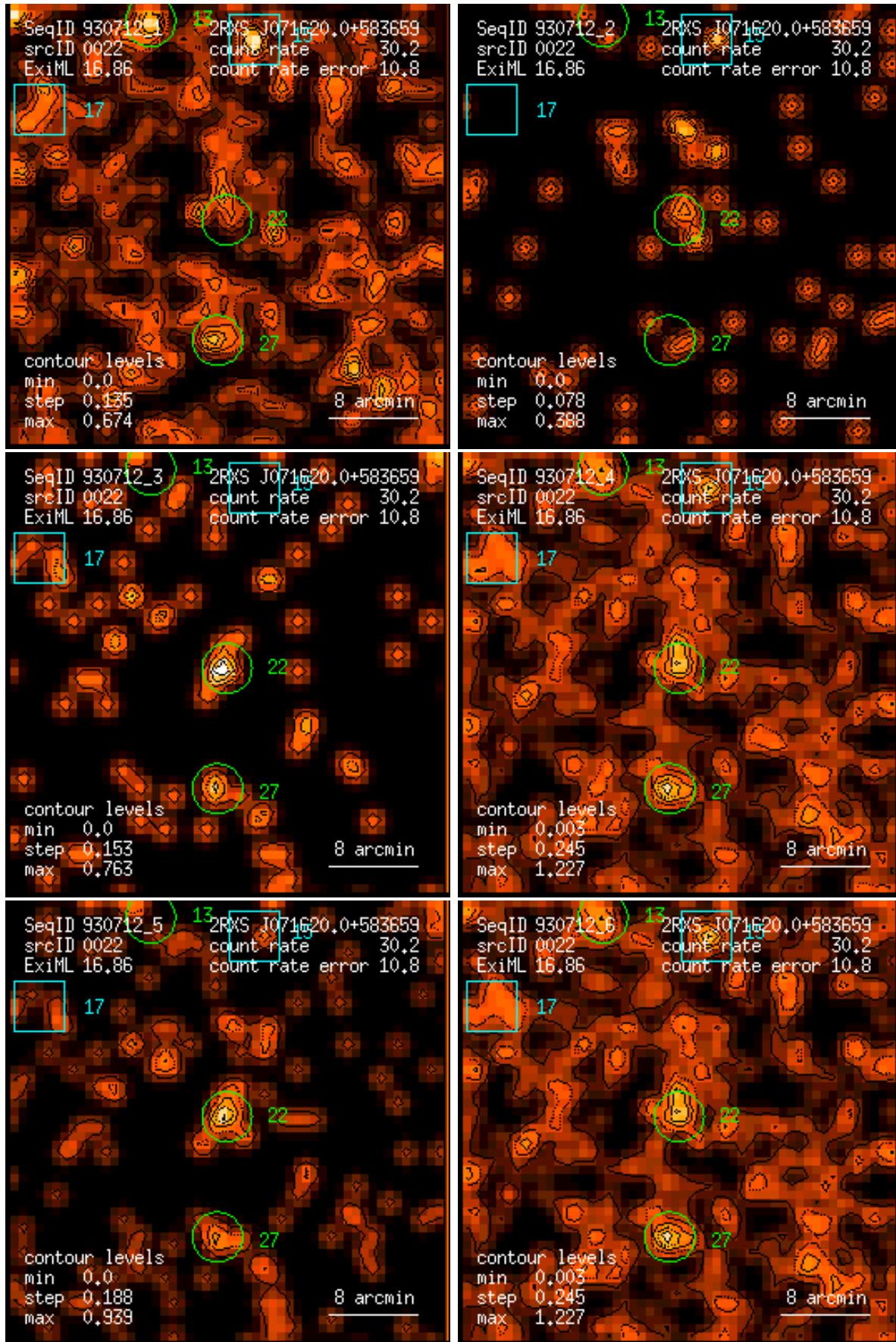
Figure 22: RASS 930712: detection 0022: band rate images, Gaussian filter: (1) PSPC channels 11 – 41, (2) 52 – 90, (3) 91 – 201, (4) 11 – 235, (5) 52 – 201, (6) 11 – 201. Broad band rates in counts/ks. Band rate contour levels in counts/ks/arcmin 2 .
