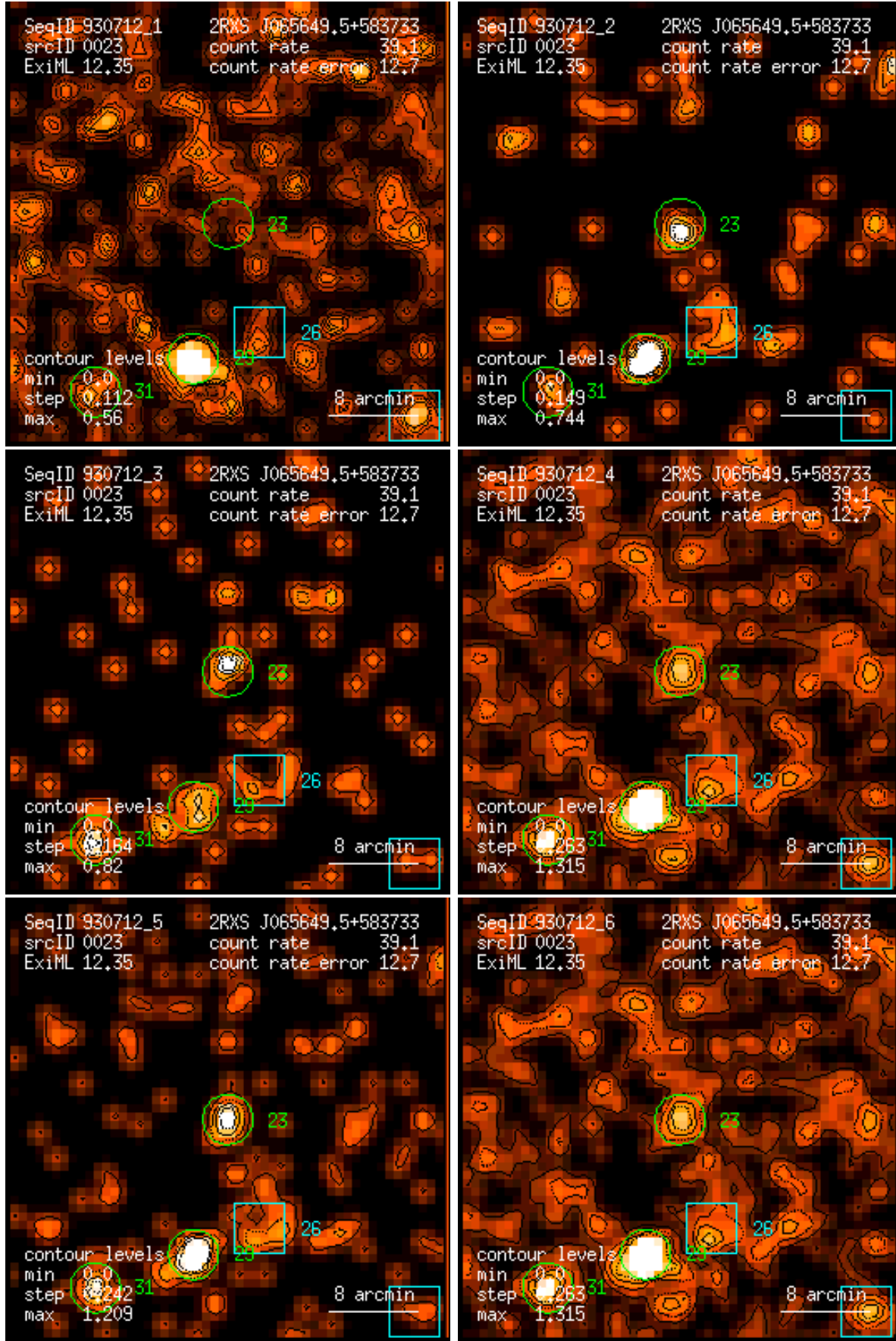
Figure 23: RASS 930712: detection 0023: band rate images, Gaussian filter: (1) PSPC channels 11 – 41, (2) 52 – 90, (3) 91 – 201, (4) 11 – 235, (5) 52 – 201, (6) 11 – 201. Broad band rates in counts/ks. Band rate contour levels in counts/ks/arcmin 2 .
