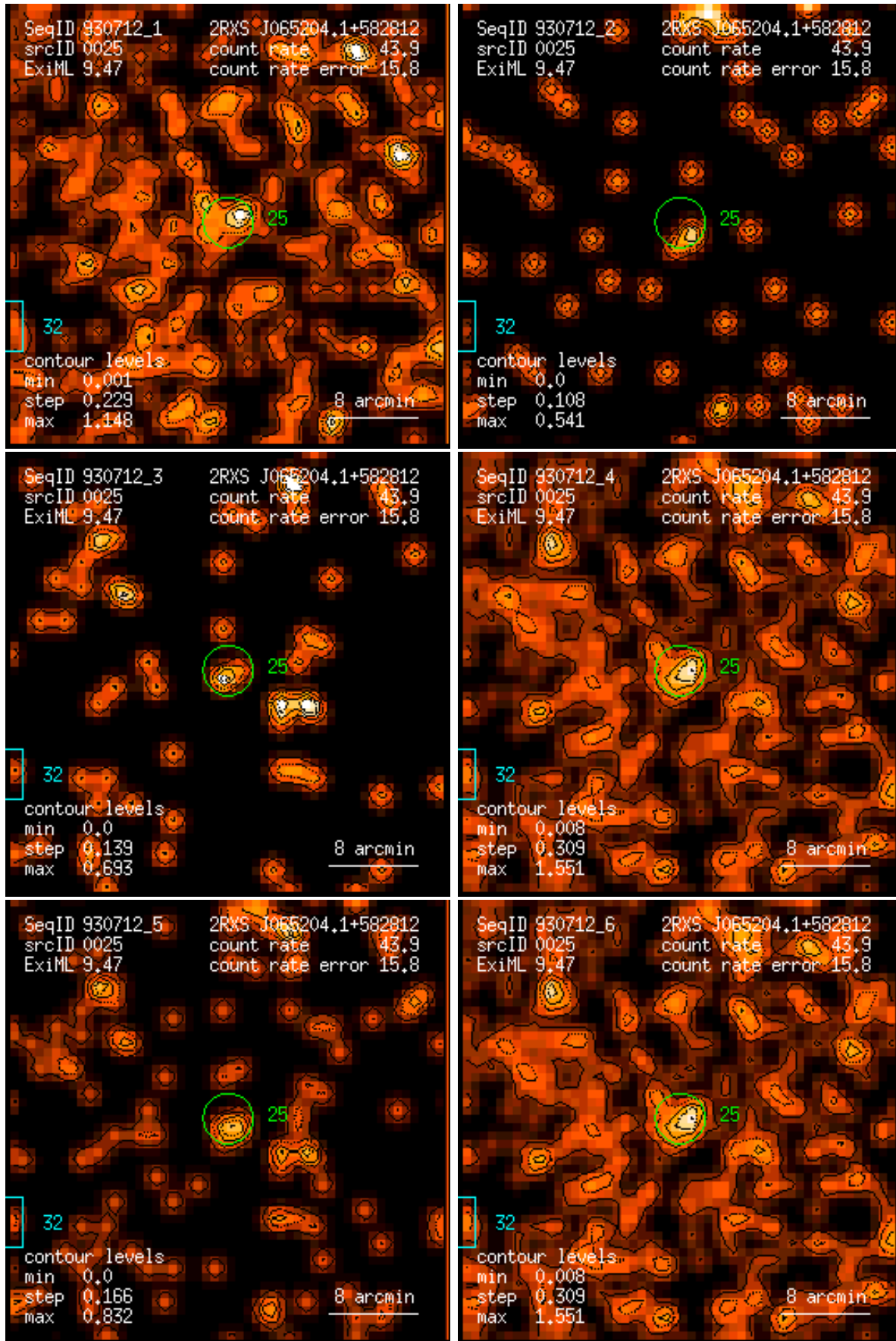
Figure 25: RASS 930712: detection 0025: band rate images, Gaussian filter: (1) PSPC channels 11 – 41, (2) 52 – 90, (3) 91 – 201, (4) 11 – 235, (5) 52 – 201, (6) 11 – 201. Broad band rates in counts/ks. Band rate contour levels in counts/ks/arcmin 2 .
