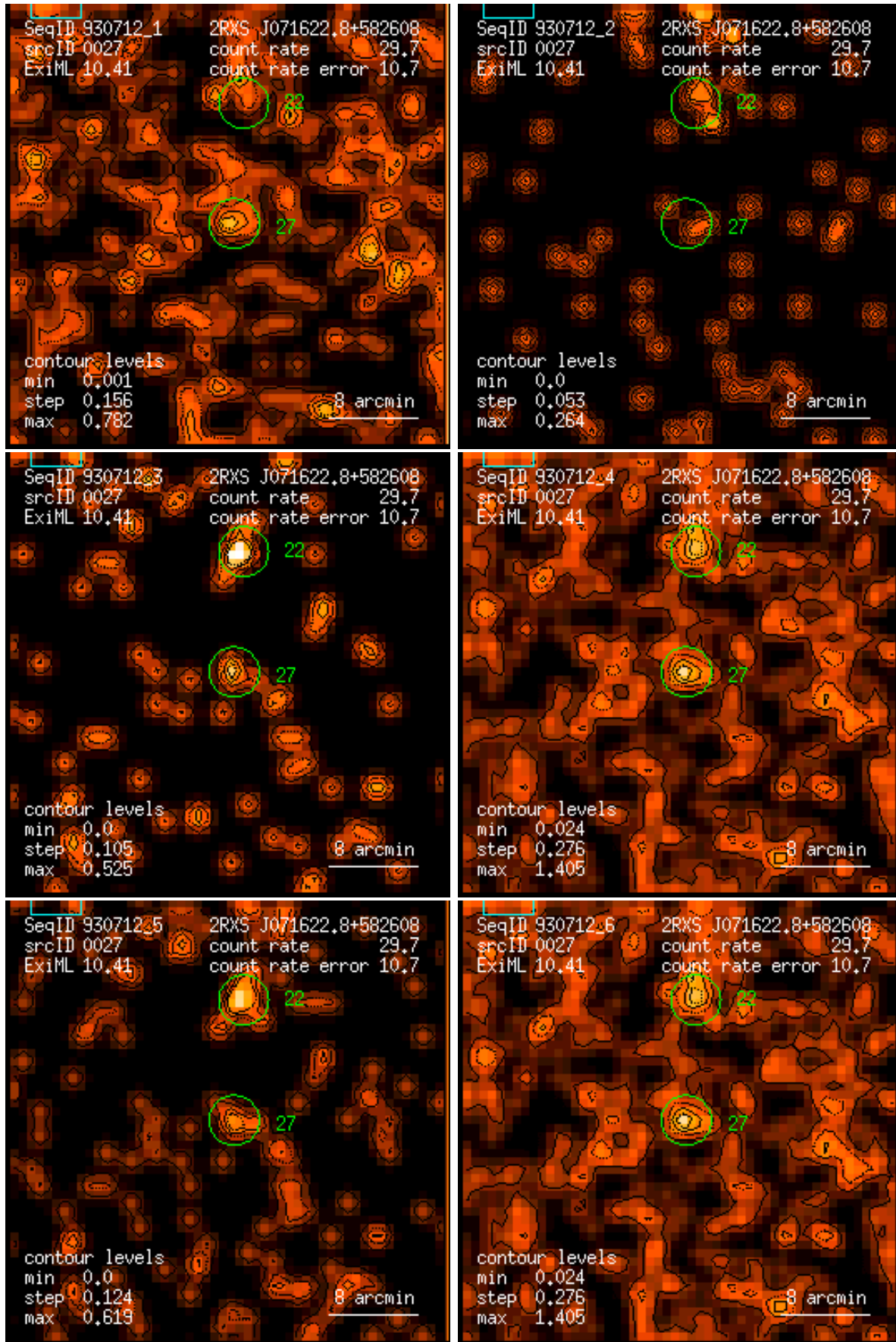
Figure 27: RASS 930712: detection 0027: band rate images, Gaussian filter: (1) PSPC channels 11 – 41, (2) 52 – 90, (3) 91 – 201, (4) 11 – 235, (5) 52 – 201, (6) 11 – 201. Broad band rates in counts/ks. Band rate contour levels in counts/ks/arcmin 2 .
