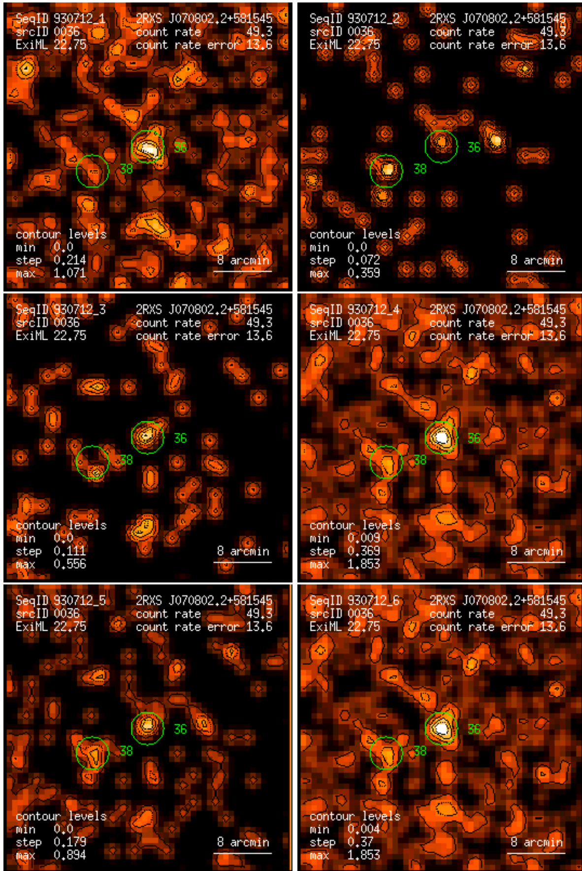
Figure 36: RASS 930712: detection 0036: band rate images, Gaussian filter: (1) PSPC channels 11 – 41, (2) 52 – 90, (3) 91 – 201, (4) 11 – 235, (5) 52 – 201, (6) 11 – 201. Broad band rates in counts/ks. Band rate contour levels in counts/ks/arcmin 2 .
