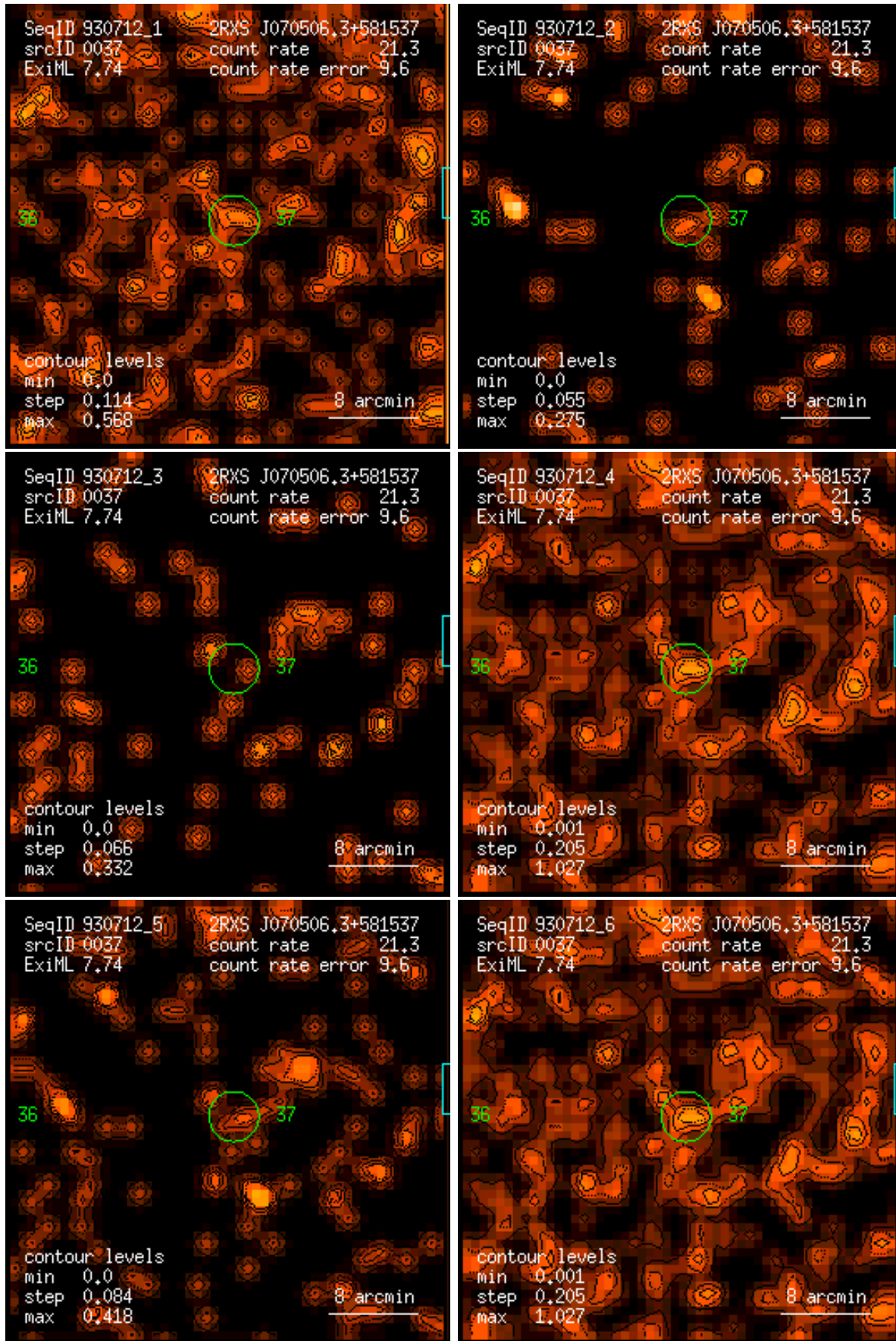
Figure 37: RASS 930712: detection 0037: band rate images, Gaussian filter: (1) PSPC channels 11 – 41, (2) 52 – 90, (3) 91 – 201, (4) 11 – 235, (5) 52 – 201, (6) 11 – 201. Broad band rates in counts/ks. Band rate contour levels in counts/ks/arcmin 2 .
