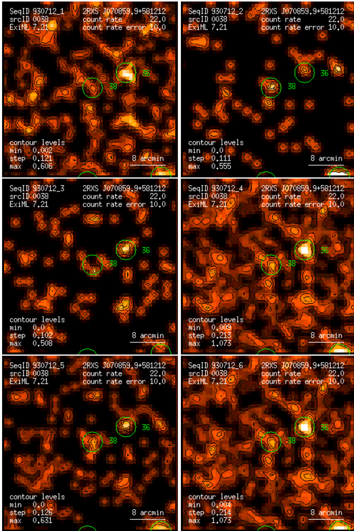
Figure 38: RASS 930712: detection 0038: band rate images, Gaussian filter: (1) PSPC channels 11 – 41, (2) 52 – 90, (3) 91 – 201, (4) 11 – 235, (5) 52 – 201, (6) 11 – 201. Broad band rates in counts/ks. Band rate contour levels in counts/ks/arcmin 2 .
