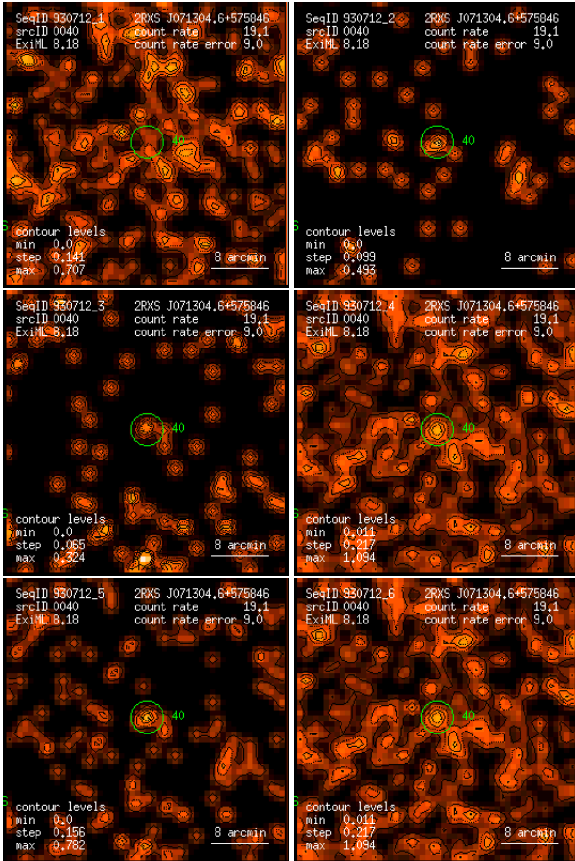
Figure 40: RASS 930712: detection 0040: band rate images, Gaussian filter: (1) PSPC channels 11 – 41, (2) 52 – 90, (3) 91 – 201, (4) 11 – 235, (5) 52 – 201, (6) 11 – 201. Broad band rates in counts/ks. Band rate contour levels in counts/ks/arcmin 2 .
