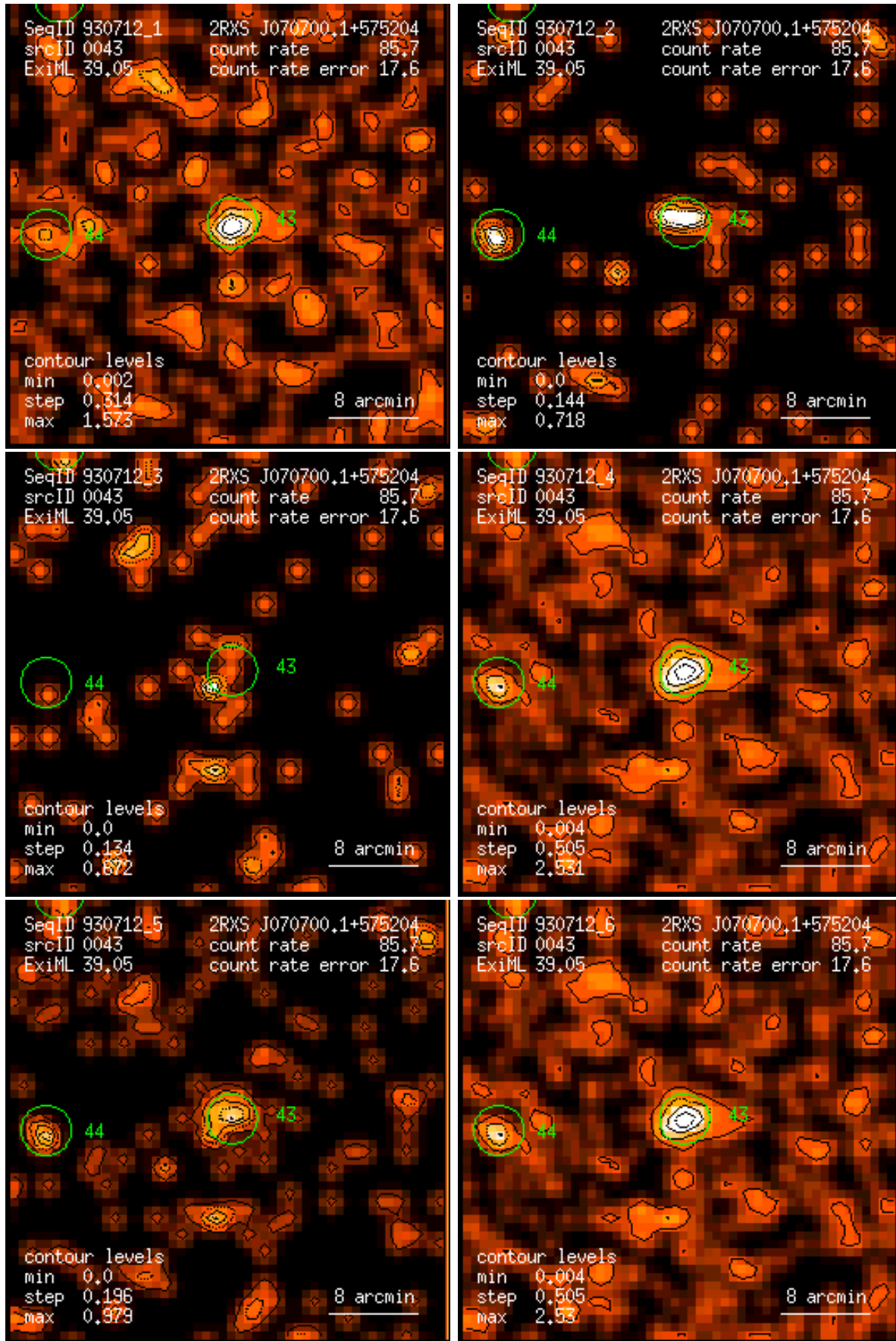
Figure 43: RASS 930712: detection 0043: band rate images, Gaussian filter: (1) PSPC channels 11 – 41, (2) 52 – 90, (3) 91 – 201, (4) 11 – 235, (5) 52 – 201, (6) 11 – 201. Broad band rates in counts/ks. Band rate contour levels in counts/ks/arcmin 2 .
