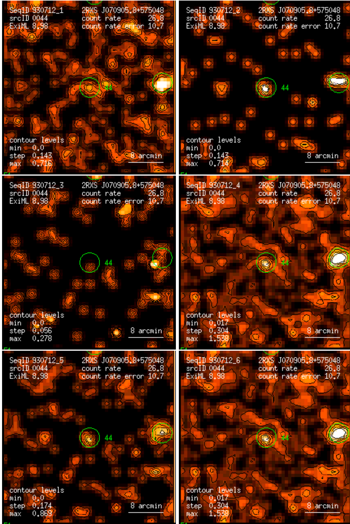
Figure 44: RASS 930712: detection 0044: band rate images, Gaussian filter: (1) PSPC channels 11 – 41, (2) 52 – 90, (3) 91 – 201, (4) 11 – 235, (5) 52 – 201, (6) 11 – 201. Broad band rates in counts/ks. Band rate contour levels in counts/ks/arcmin 2 .
