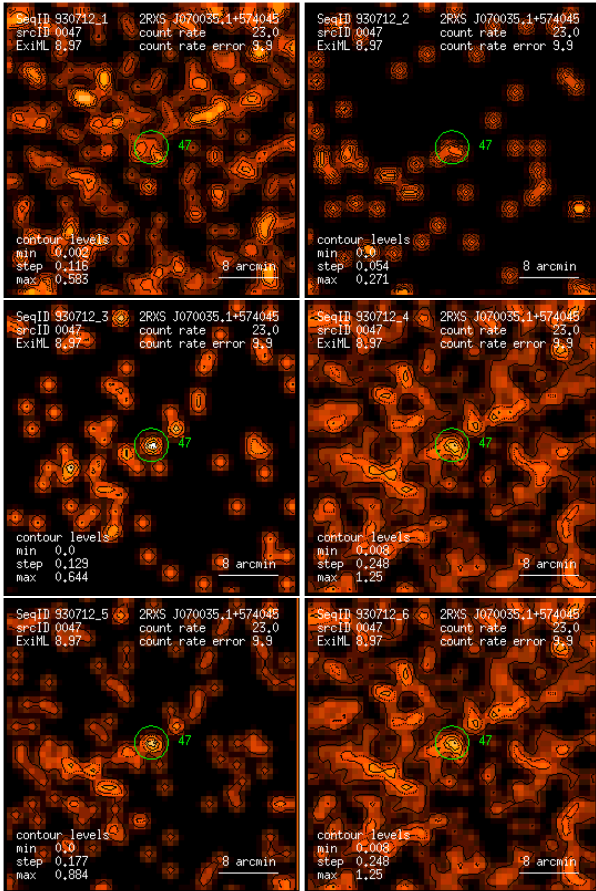
Figure 47: RASS 930712: detection 0047: band rate images, Gaussian filter: (1) PSPC channels 11 – 41, (2) 52 – 90, (3) 91 – 201, (4) 11 – 235, (5) 52 – 201, (6) 11 – 201. Broad band rates in counts/ks. Band rate contour levels in counts/ks/arcmin 2 .
